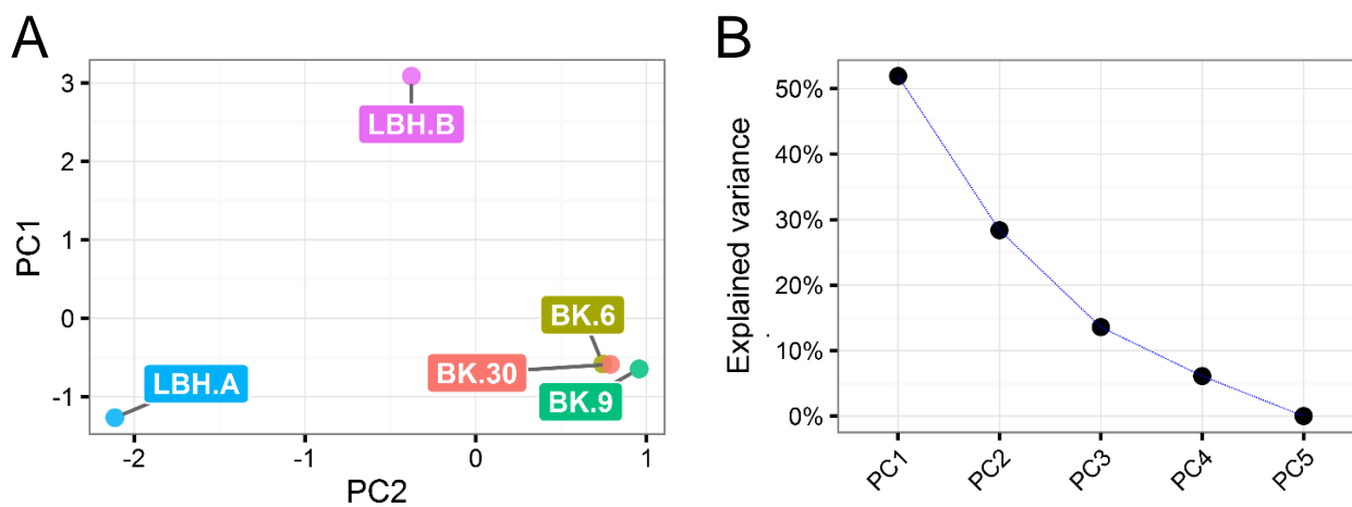
Fig. S3. Principal component analysis (PCA) conducted with moderate- and high-impact variants predicted within samples of each type. The analysis clearly separated field isolates and laboratory strains of the same type (A), with ~80% of the variability from each class explained by the first two principal components (B).
