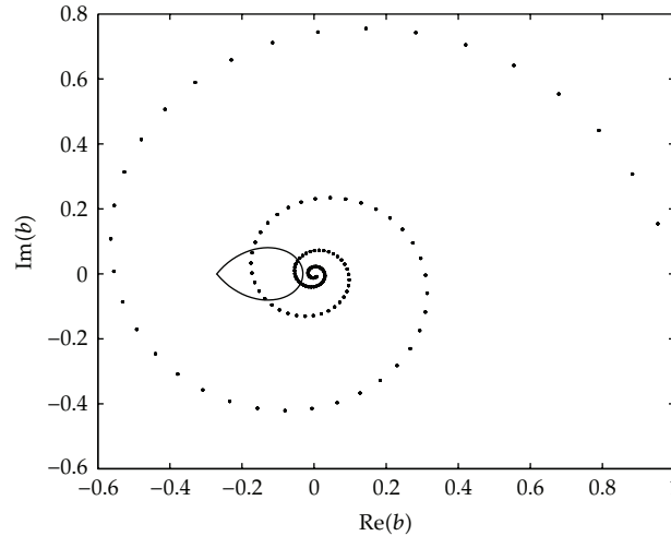
Figure 6: The stability oval and points M^{(s)} for Example 6.1.
