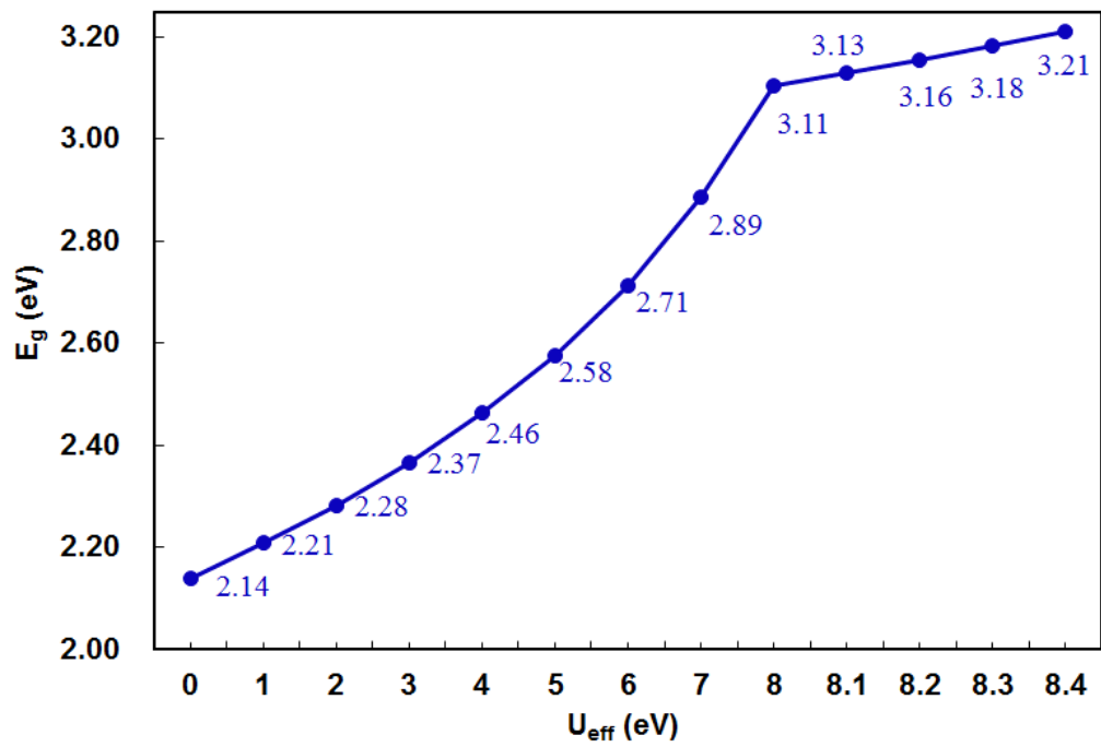
Figure S1: Relationship between the effective Hubbard parameter ( U_{\text{eff}} ) and the band gap ( E_g ) of anatase \text{TiO}_2 .
