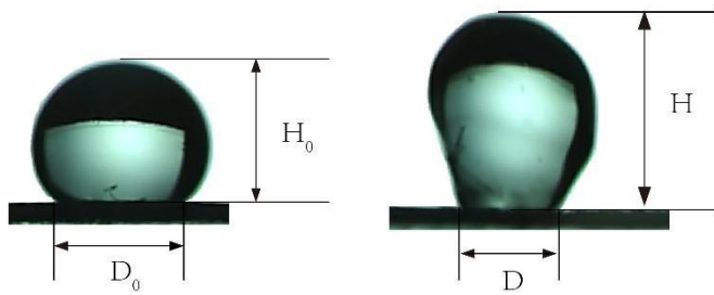
Fig. S2 The contact line and contact height of droplet before and after vertical vibration
