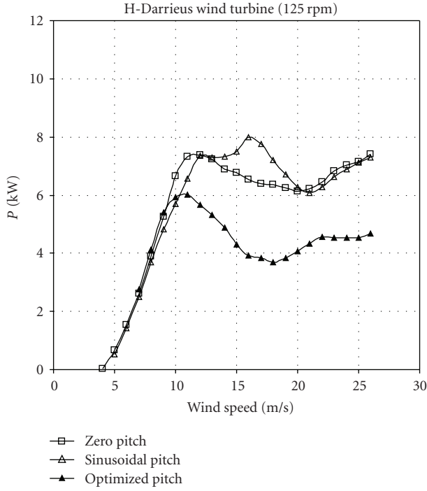
FIGURE 7: Power versus wind speed for the 7 kW VAWT with fixed and optimized variable pitch.
