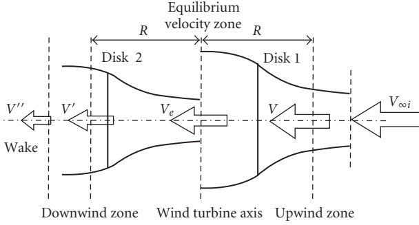
FIGURE 1: The two actuator disks model.
