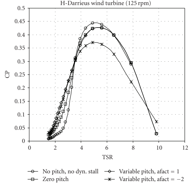
FIGURE 4: Power coefficient versus TSR for the 7 kW VAWT with fixed and variable pitch blades.
