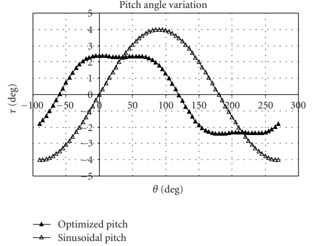
FIGURE 5: Optimal variation of the blade pitch angle.
