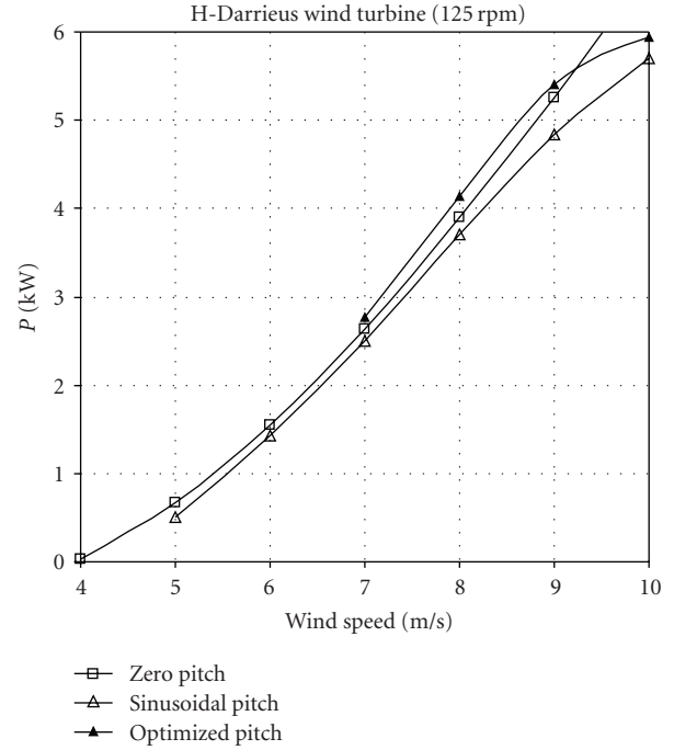
FIGURE 8: Power versus wind speed for the 7 kW VAWT with fixed and optimized variable pitch (detail).
