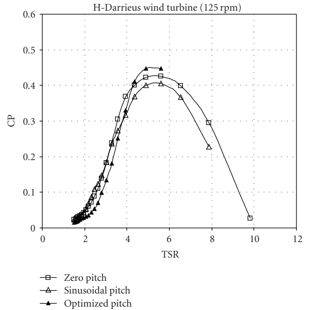
FIGURE 6: Power coefficient versus TSR for the 7 kW VAWT with fixed and optimized variable pitch.
