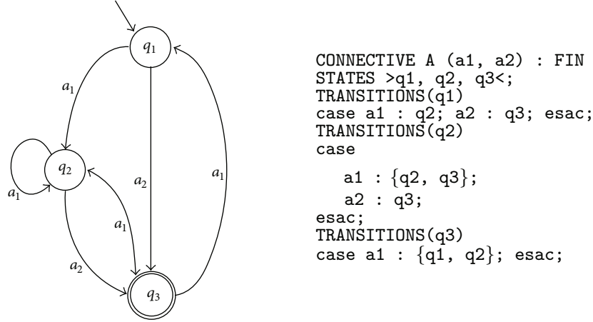
FIGURE 1: An automata connective declaration in ENuSMV.
