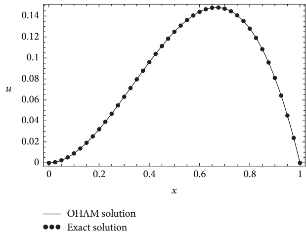
FIGURE 1: Exact and approximate solution using OHAM for Example 1.
