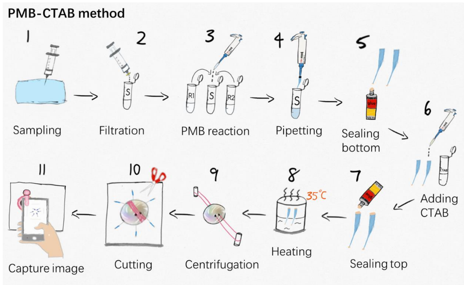
Figure S1. Schematic illustration of field preconcentration and digital image colorimetric sensing of phosphate by the PMB-CTAB method.
