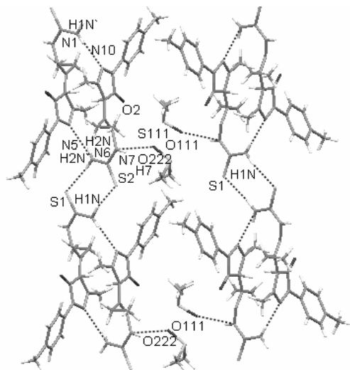
Figure 3. Packing of PropPTMP-ths forming cavity
