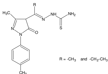
Figure 1. Pyrazolone thiosemicarbazone
