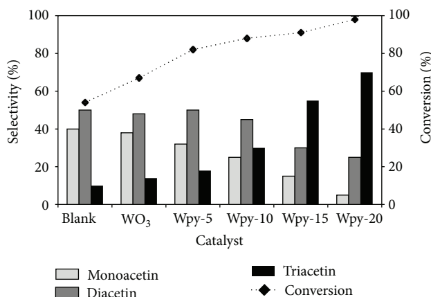
FIGURE 12: Influence of \text{WO}_3 loading on conversion and selectivity. (Reaction temperature: 110^\circ\text{C} ; reaction time: 10 h; catalyst weight: 0.4 g; AcOH/Gly mole ratio: 6.)
