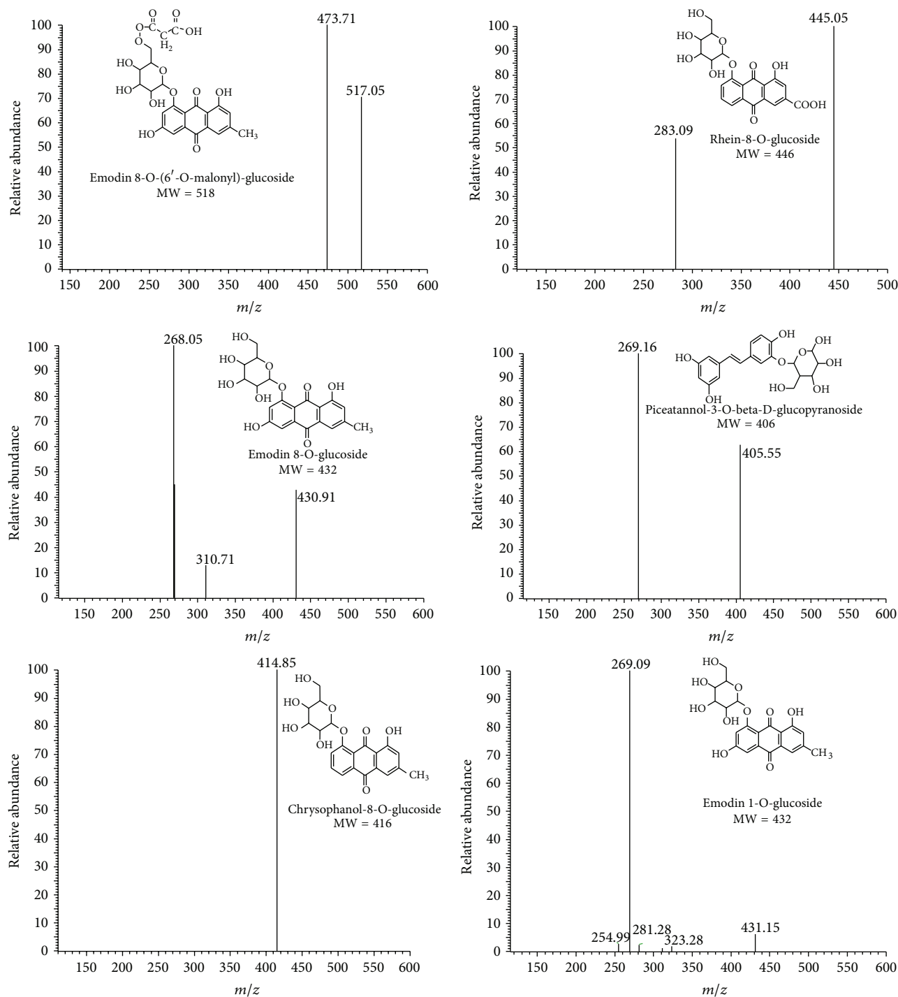
FIGURE 4: ESI-MS/MS of rhubarb anthraquinone glucosides.
