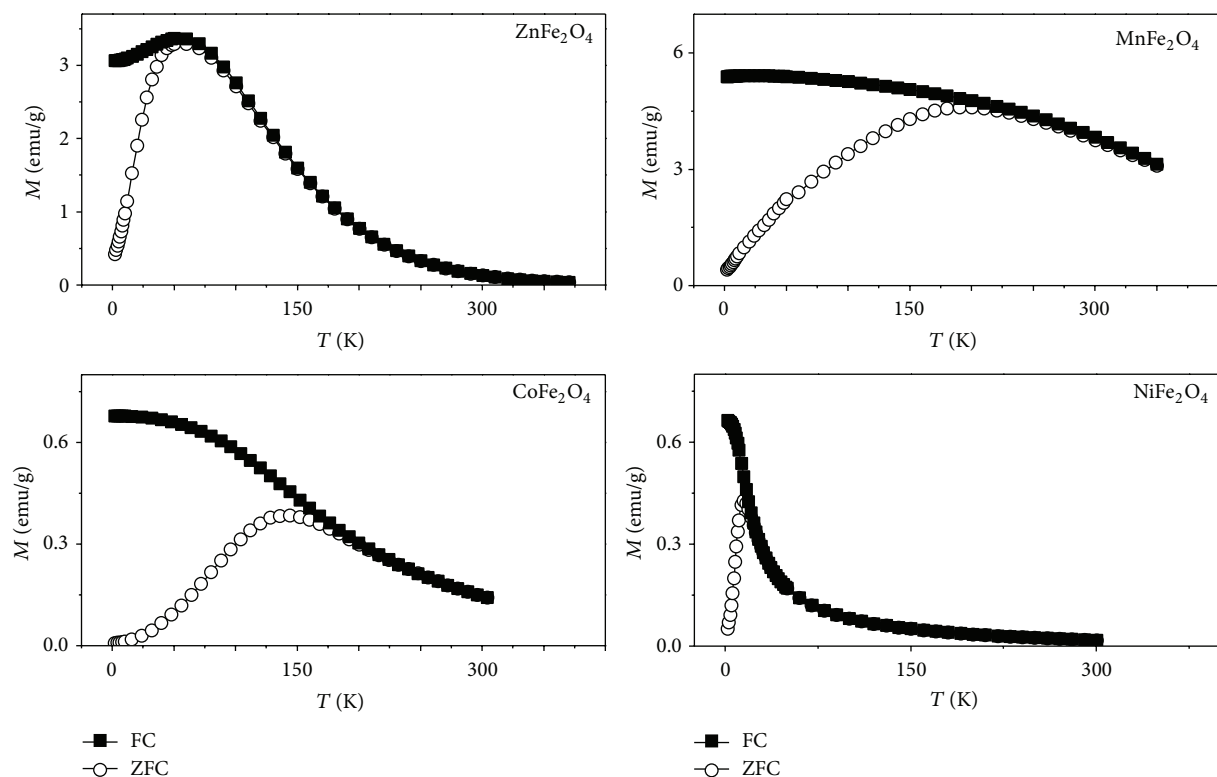
FIGURE 5: Temperature dependences of magnetization M (ZFC- and FC-measurements) for the NPs of zinc, manganese, cobalt, and nickel spinel ferrites. Measurements were carried out in magnetic field H_{\text{measur}} = 20 Oe.
