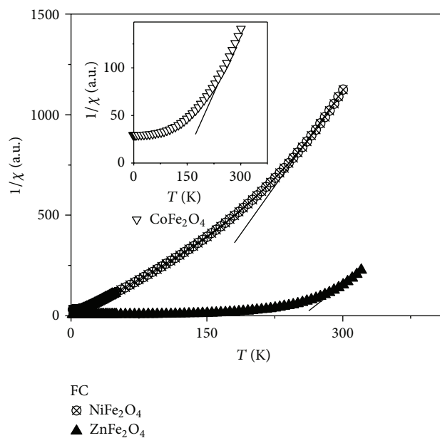
FIGURE 6: Temperature dependences of reciprocal susceptibility \chi^{-1}(T) for the NPs of zinc, cobalt, and nickel spinel ferrites.
