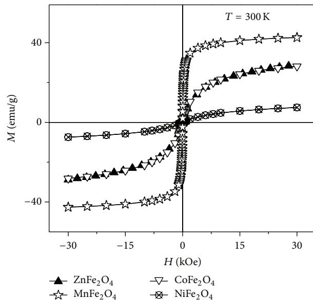
FIGURE 7: The magnetization M versus magnetic field H dependences for the NPs of zinc, manganese, cobalt, and nickel spinel ferrites. The magnetization curves were obtained at 300 K.
