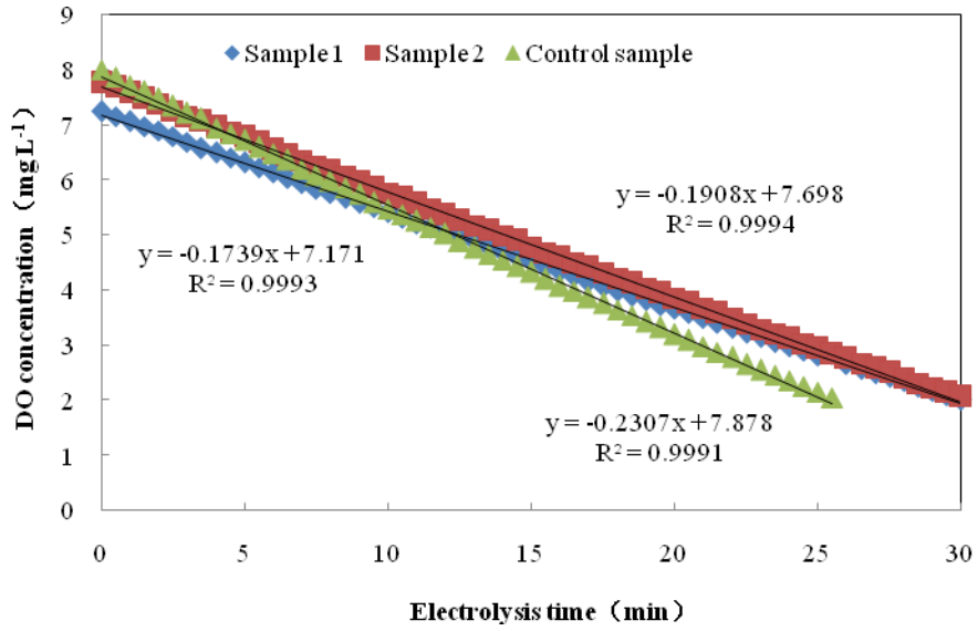
FIGURE S1: OUR of activated sludge at electrolysis time of 15 min
