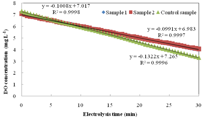
FIGURE S2: OUR of activated sludge at electrolysis time of 30 min
