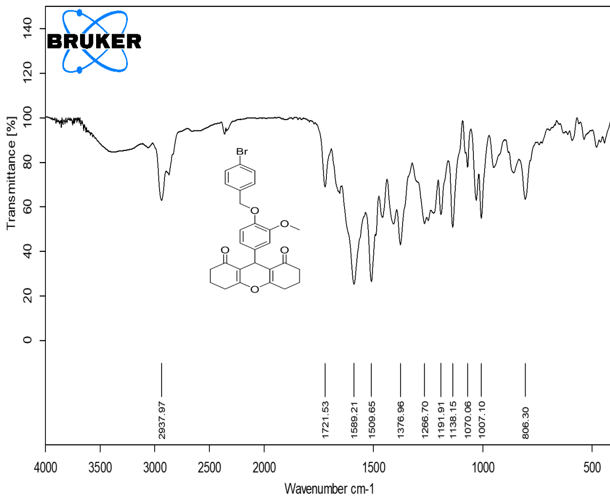
IR spectrum of 4j
