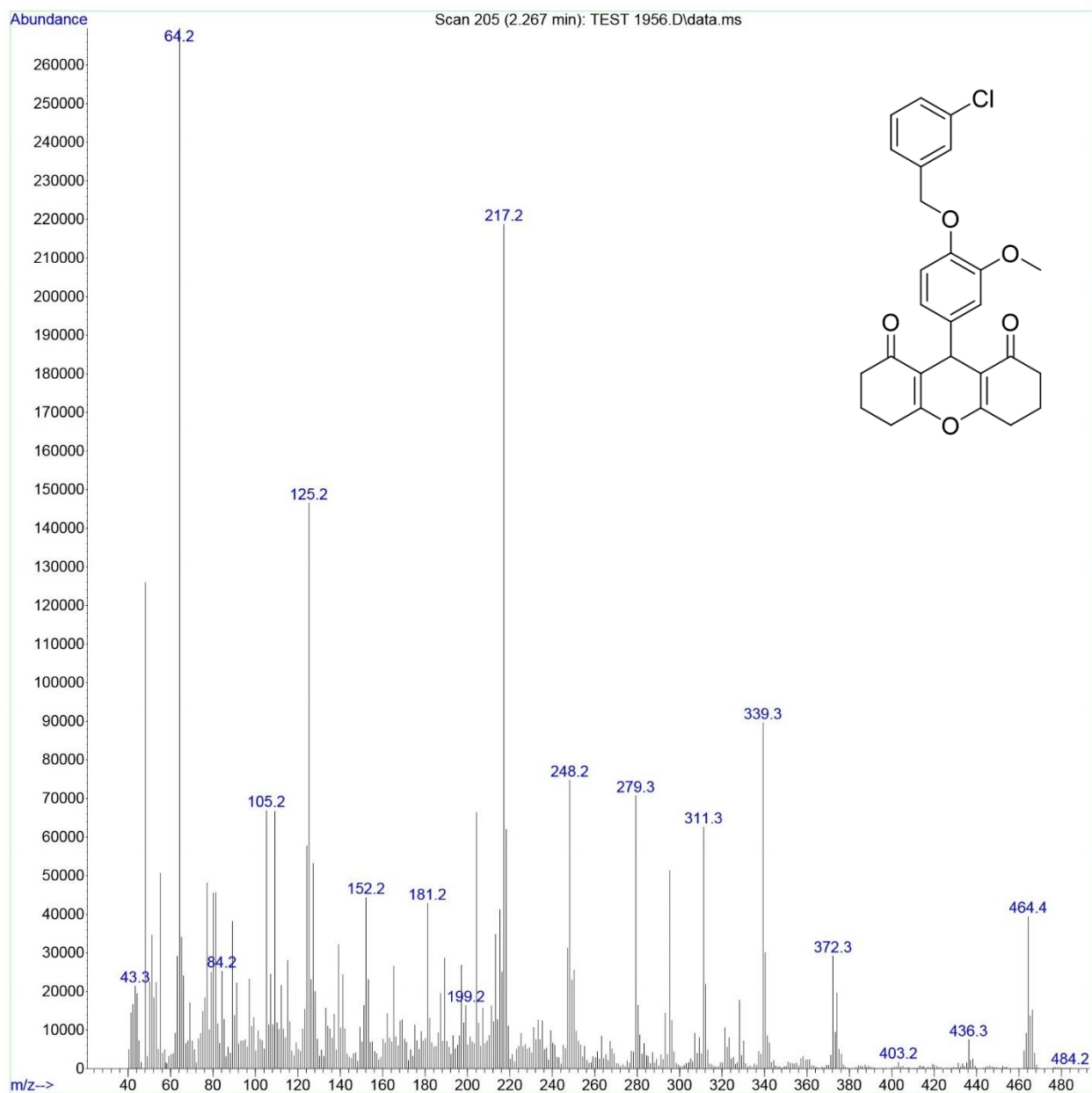
Mass spectrum of 4k
