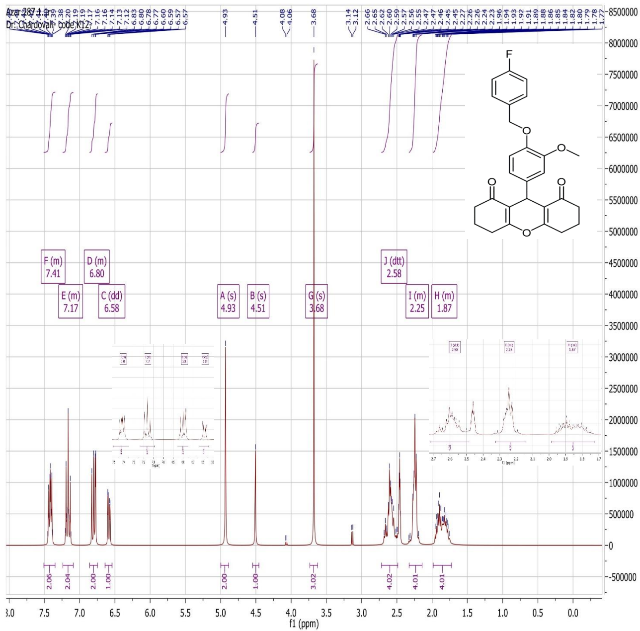
1 H-NMR spectrum of 4I
