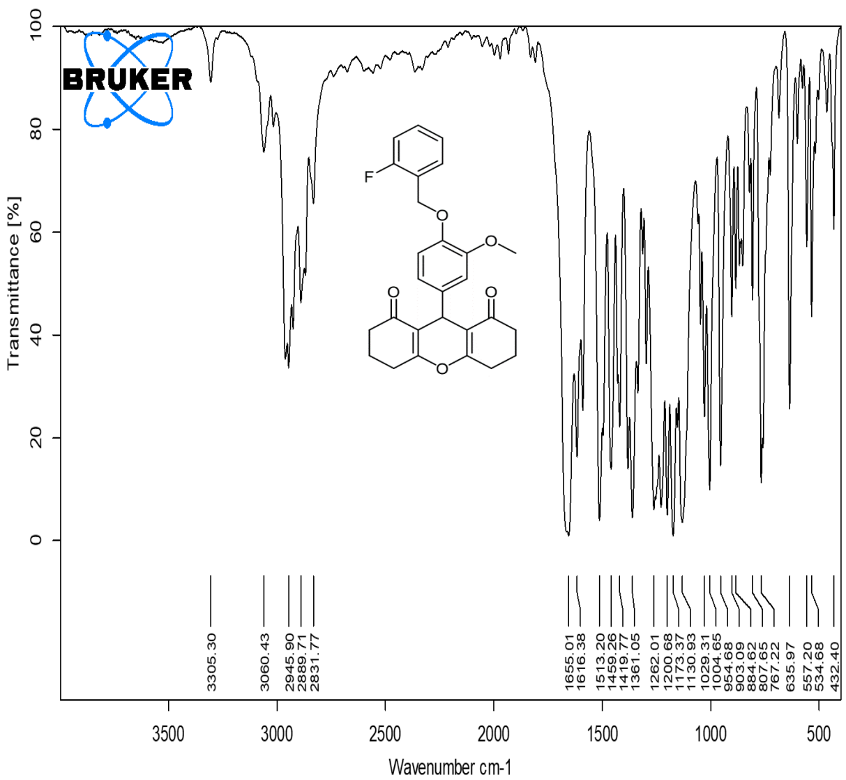
IR spectrum of 4m
