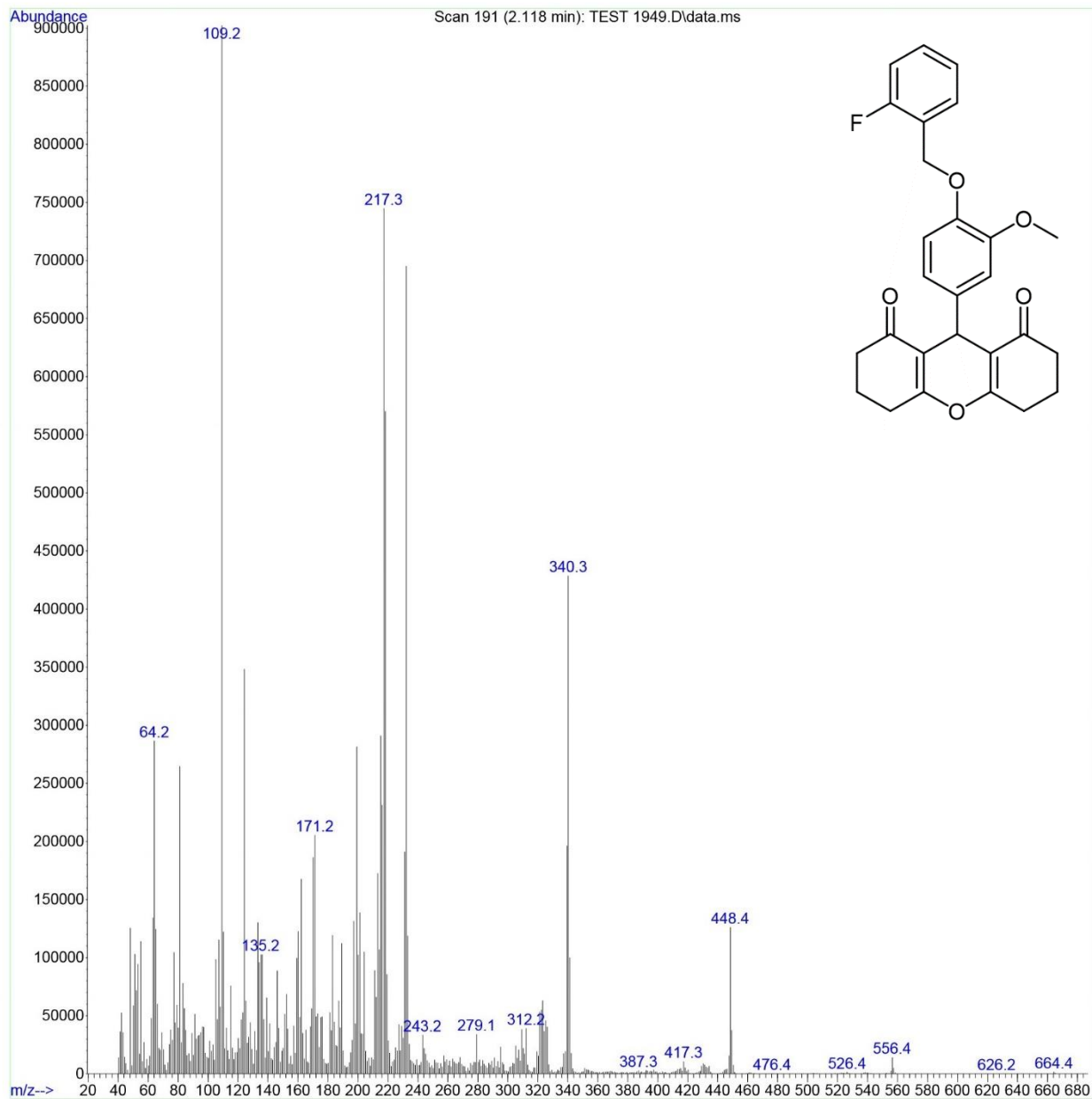
Mass spectrum of 4m
