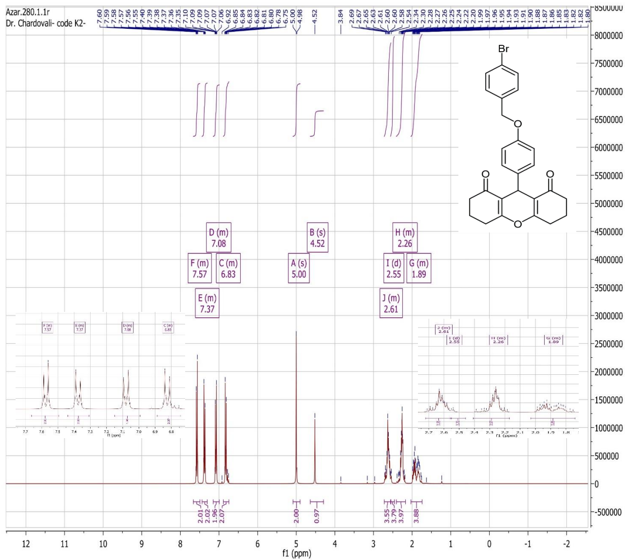
1 H-NMR spectrum of 4b
