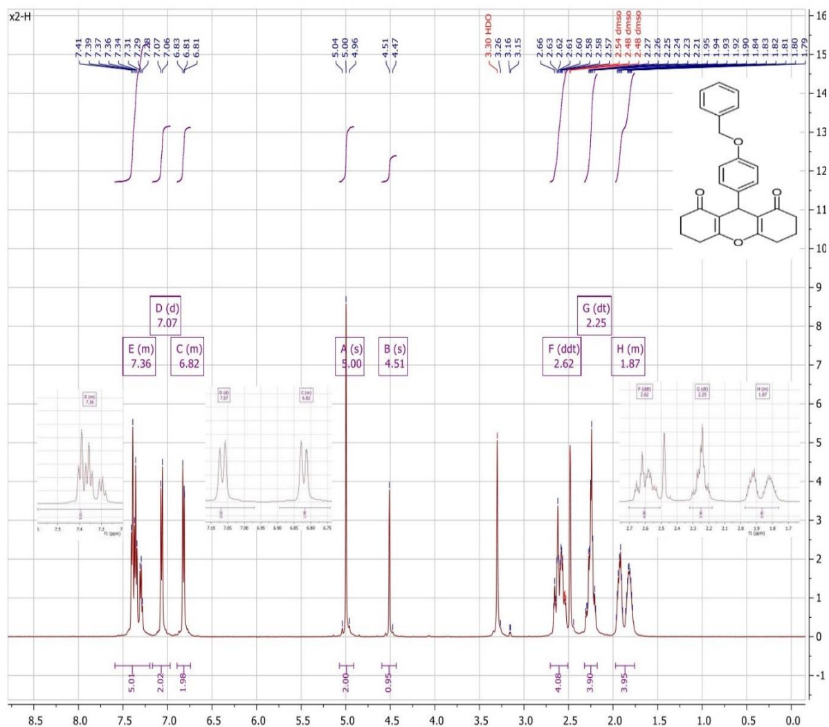
1 H-NMR spectrum of 4a
