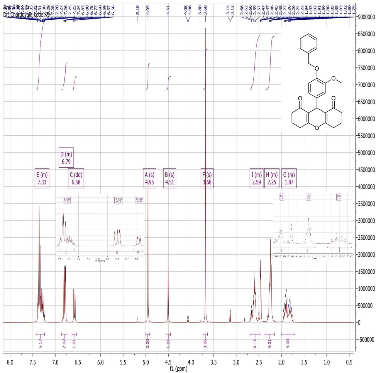
^1\text{H-NMR} spectrum of 4i
