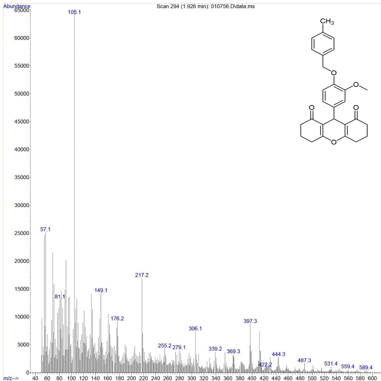
Mass spectra of 4o
