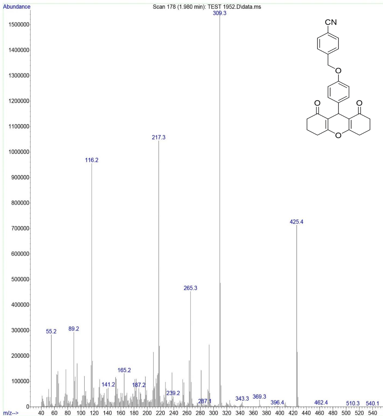
Mass spectrum of 4q
