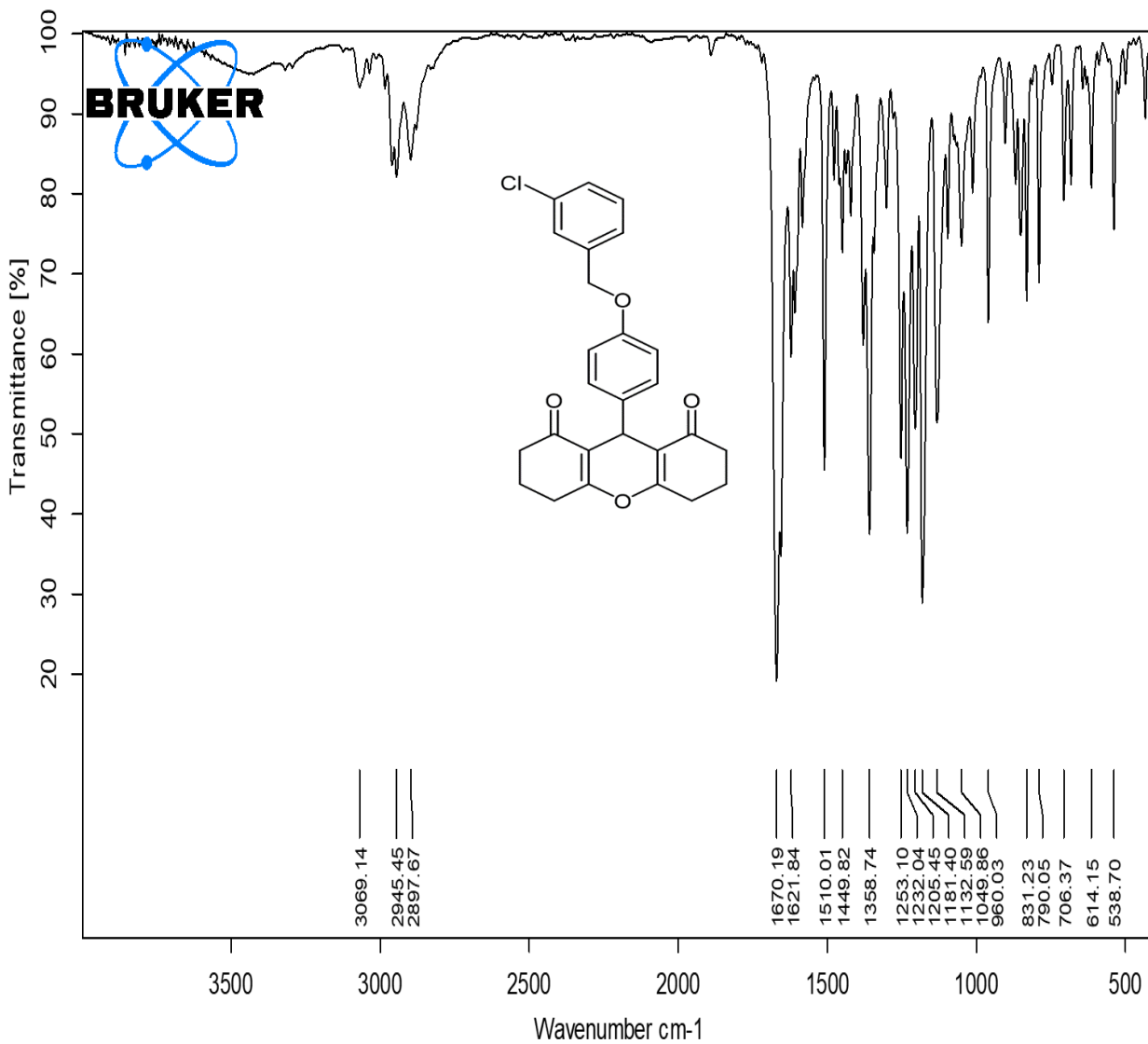
IR spectrum of 4c
