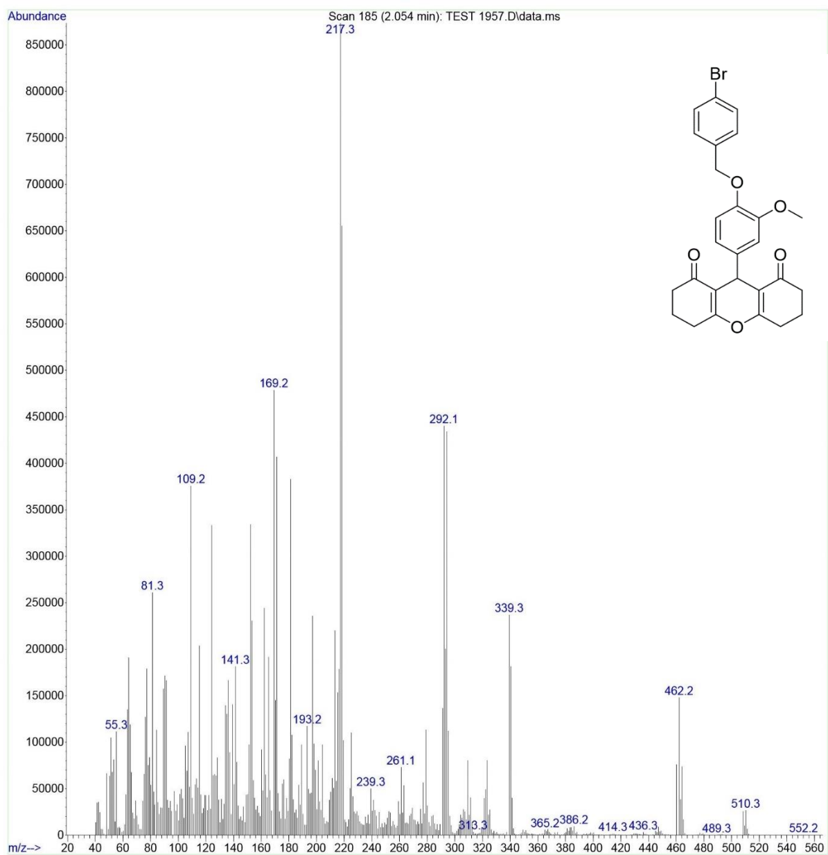
Mass spectrum of 4j
