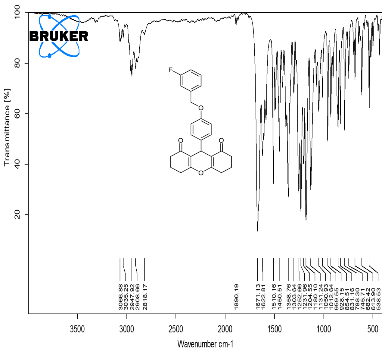
IR spectrum of 4f
