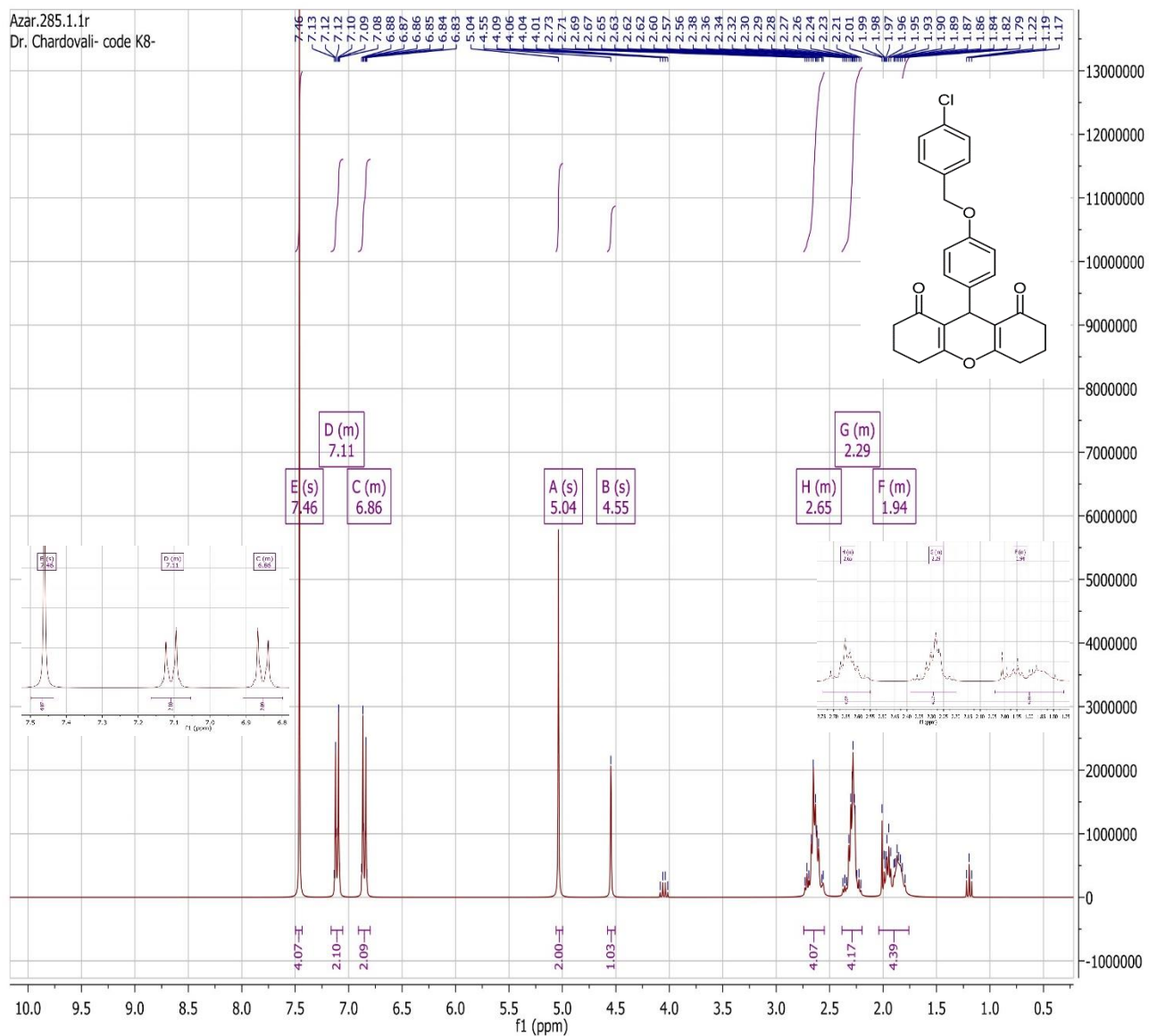
1 H-NMR spectrum of 4h
