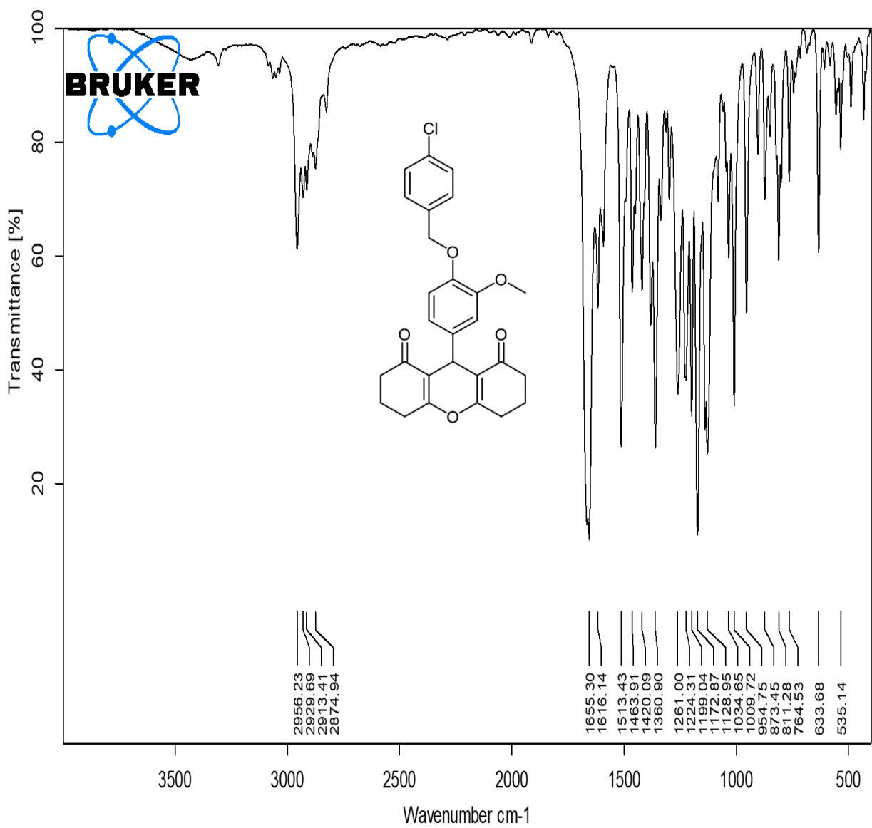
IR spectrum of 4p
