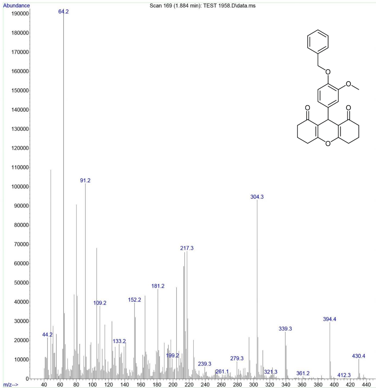
Mass spectrum of 4i
