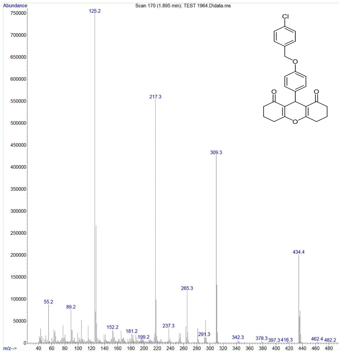
Mass spectrum of 4h
