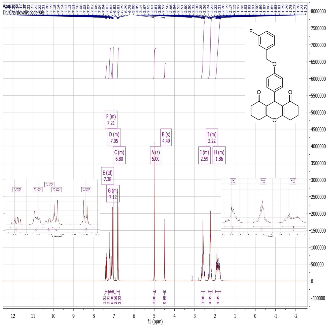
1 H-NMR spectrum of 4f
