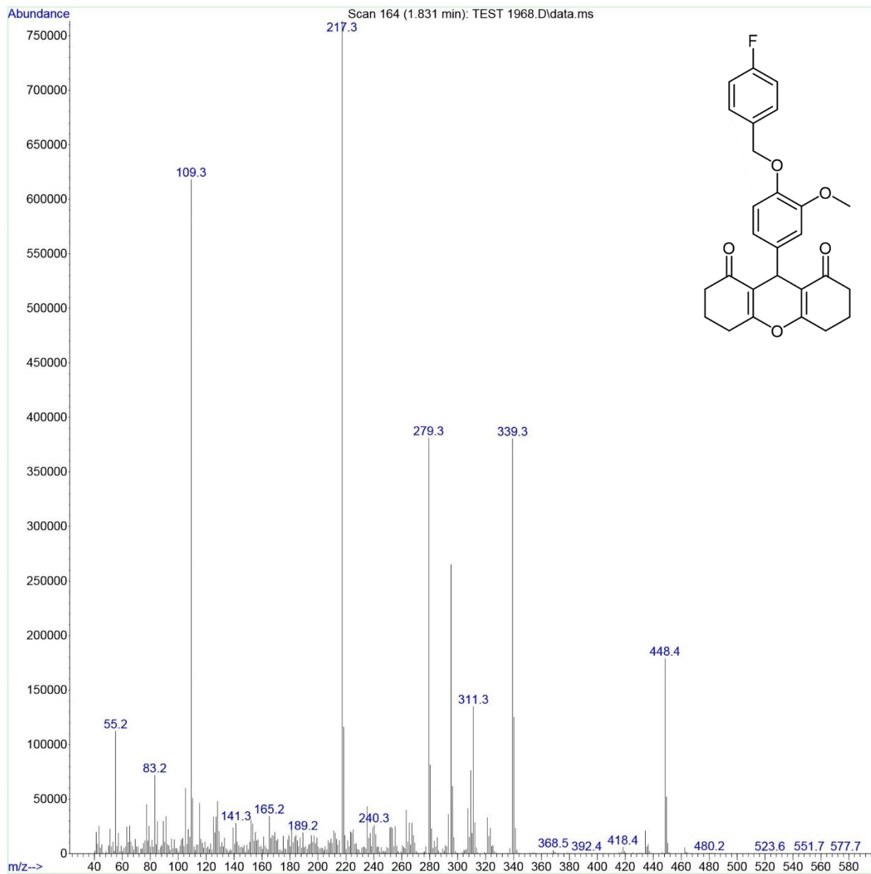
Mass spectrum of 4I
