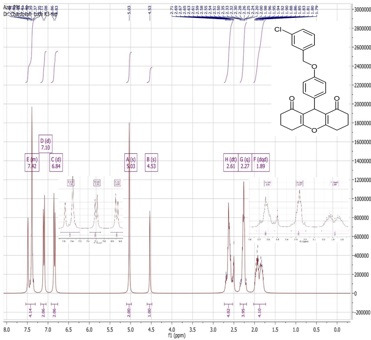
1 H-NMR spectrum of 4c
