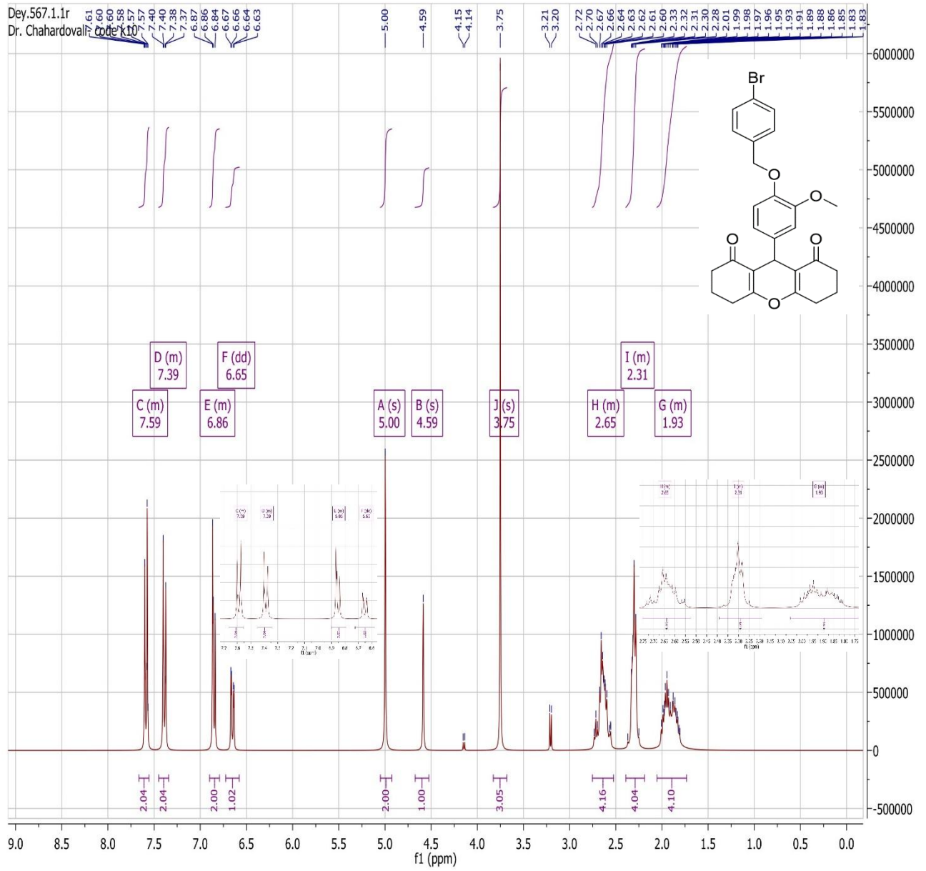
1 H-NMR spectrum of 4j
