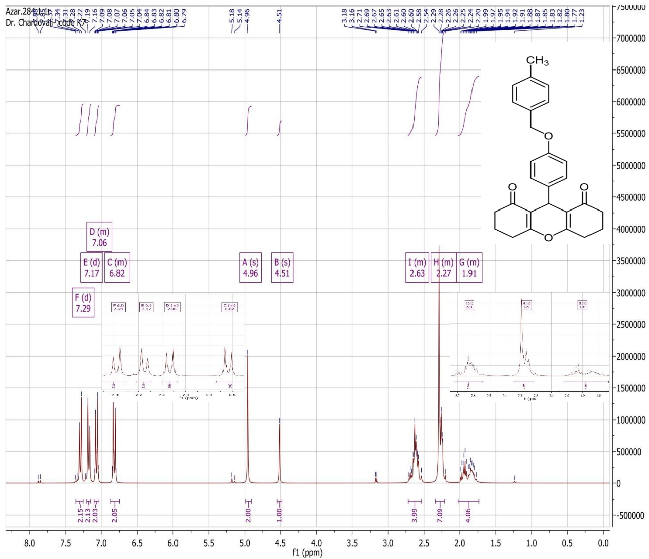
1 H-NMR spectrum of 4g
