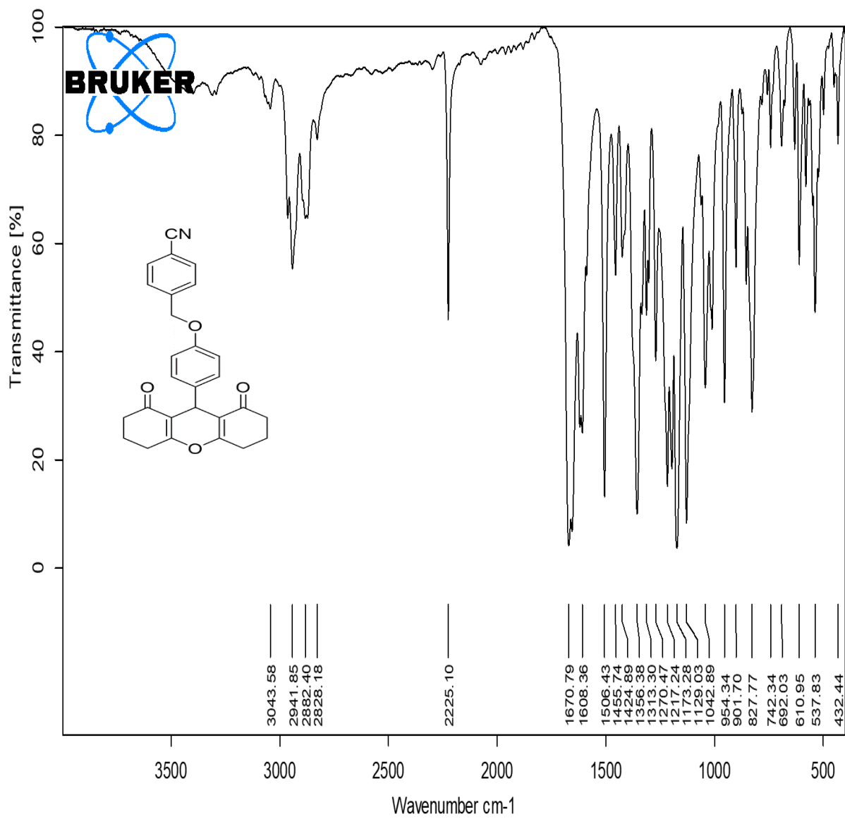
IR spectrum of 4q
