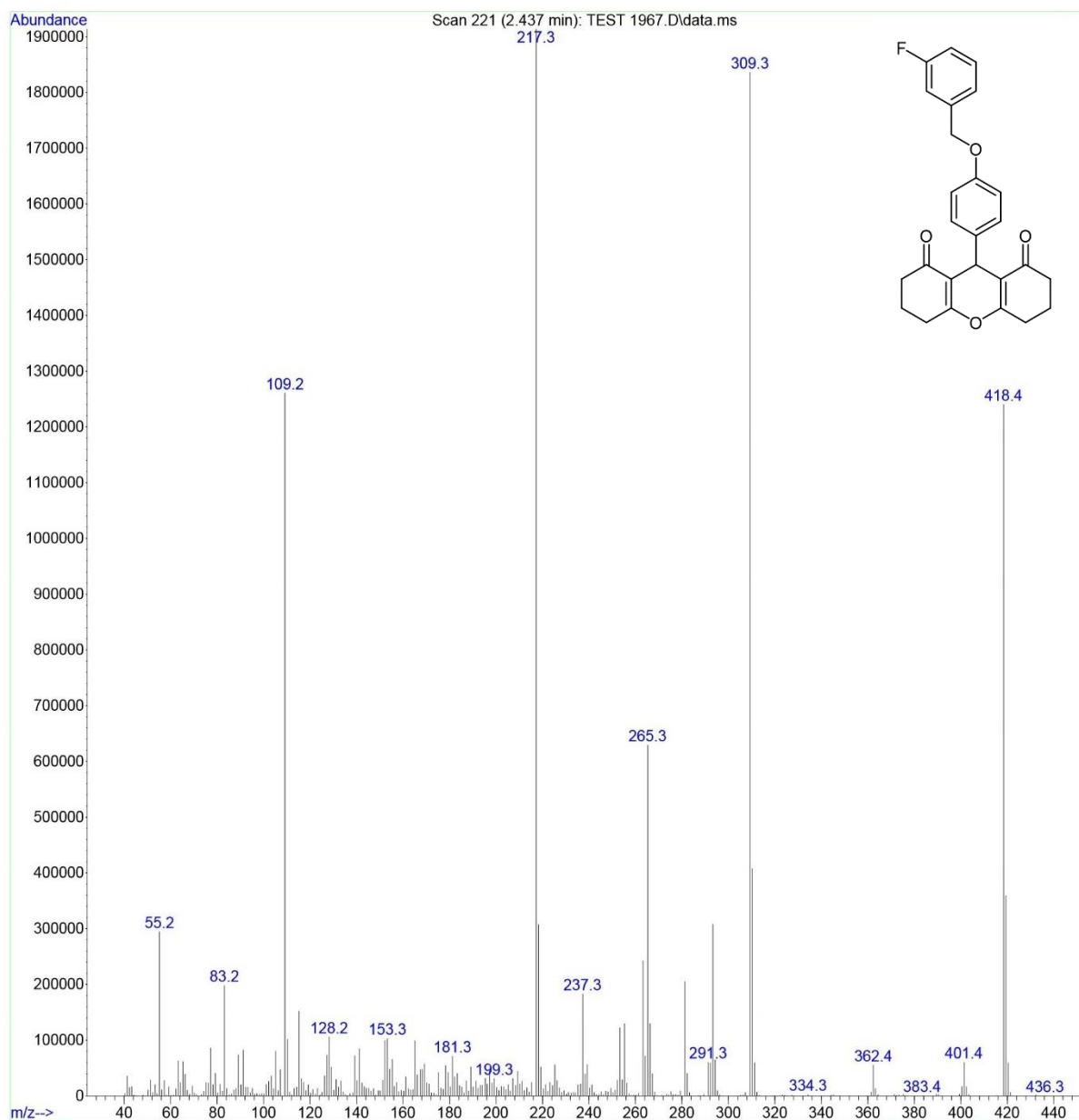
Mass spectrum of 4f
