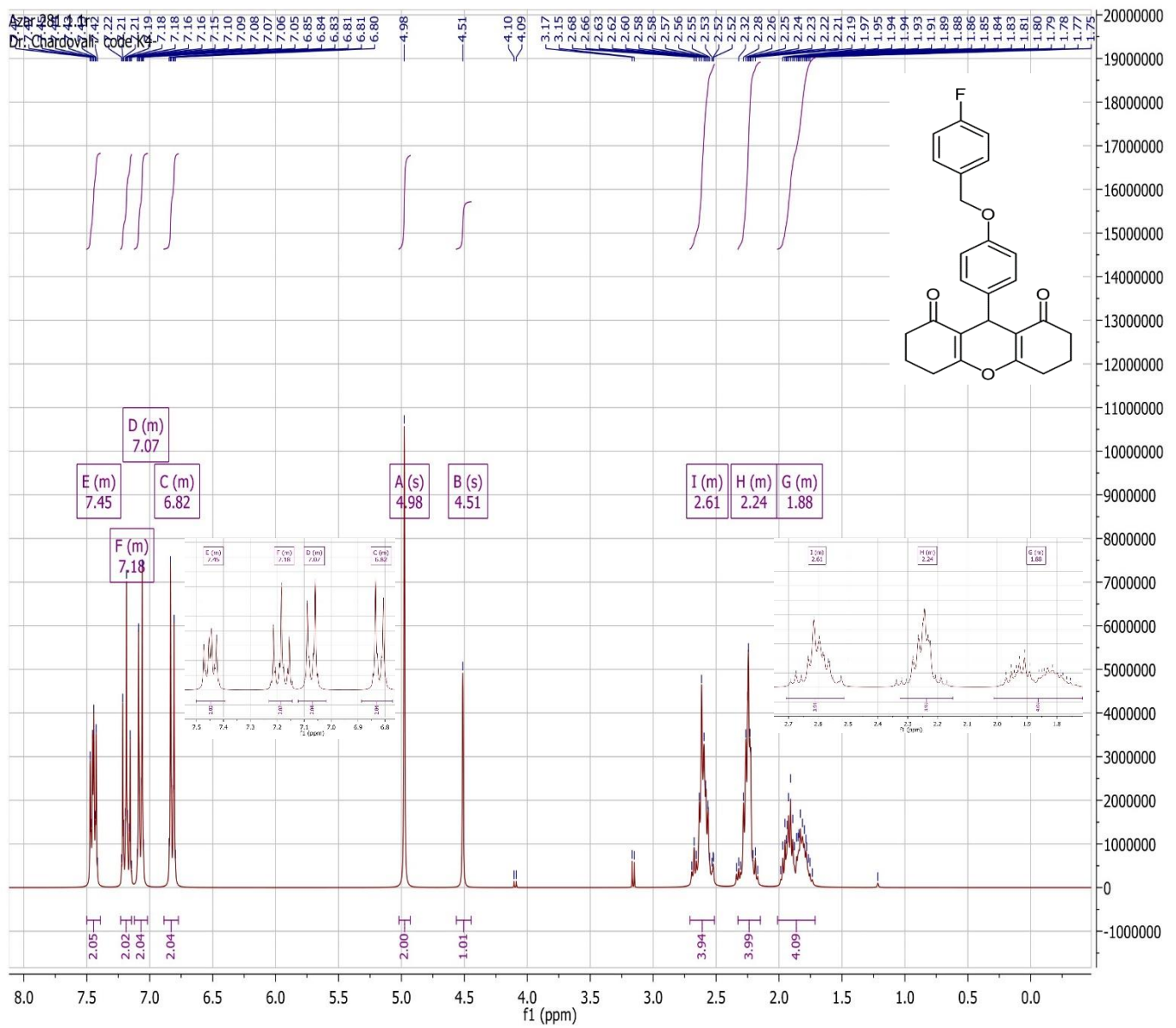
1 H-NMR spectrum of 4d
