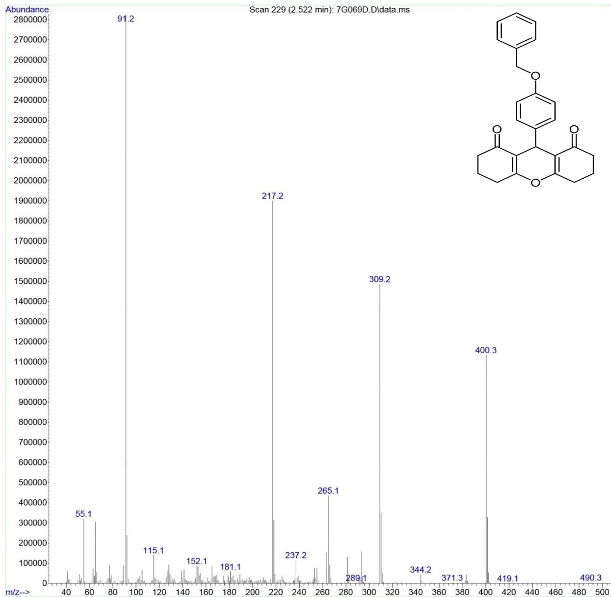
Mass spectrum of 4a
