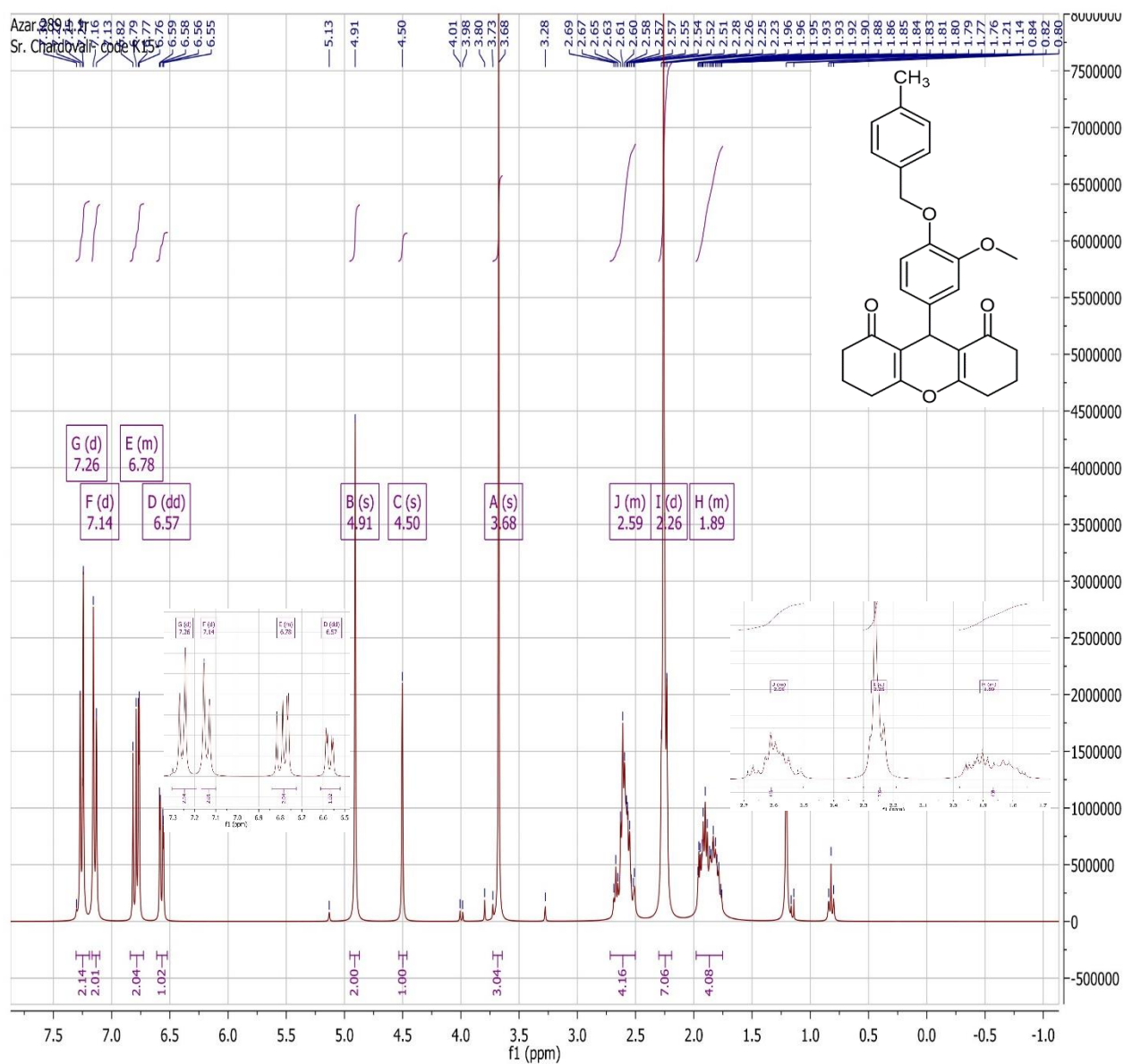
1 H-NMR spectrum of 4o
