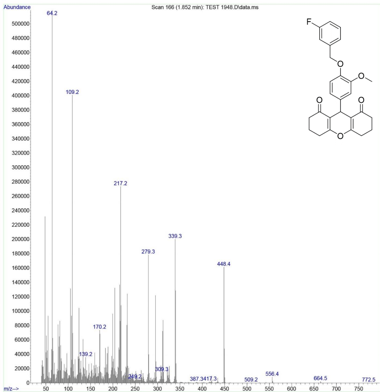
Mass spectrum of 4n
