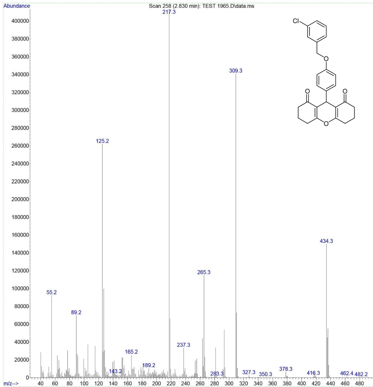
Mass spectrum of 4c
