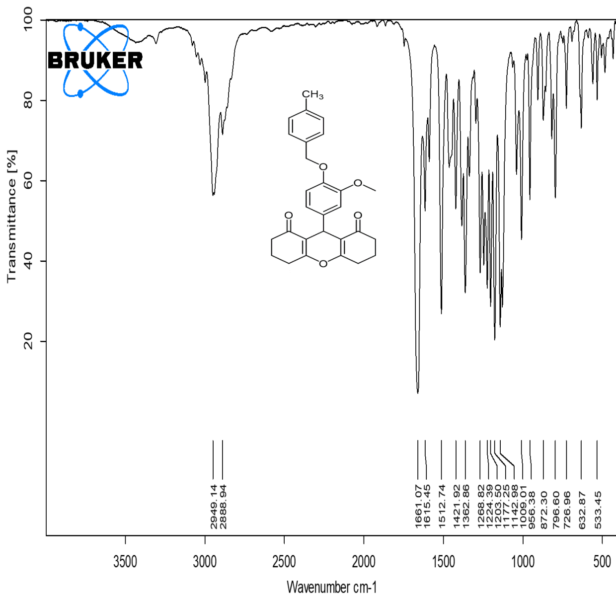
IR spectrum of 4o
