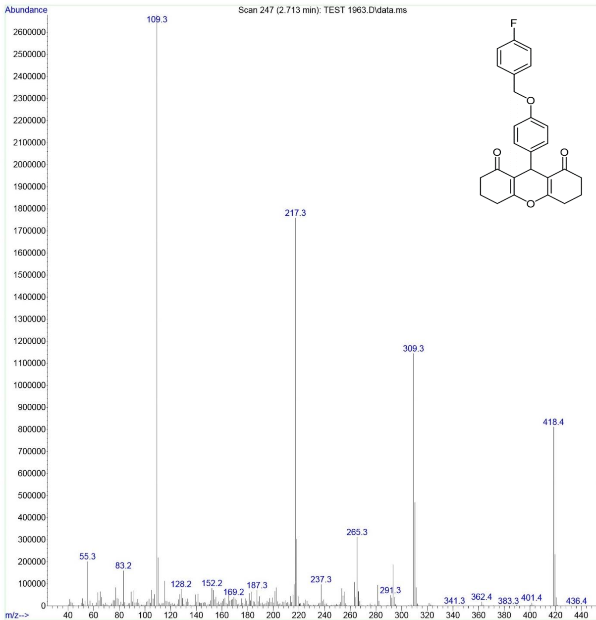
Mass spectrum of 4d
