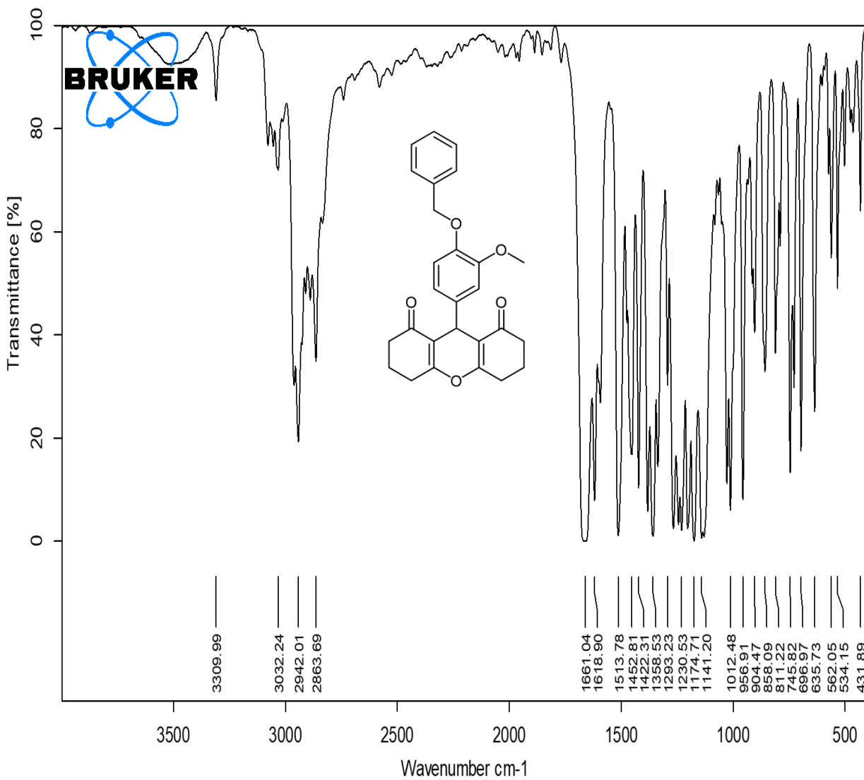
IR spectrum of 4i
