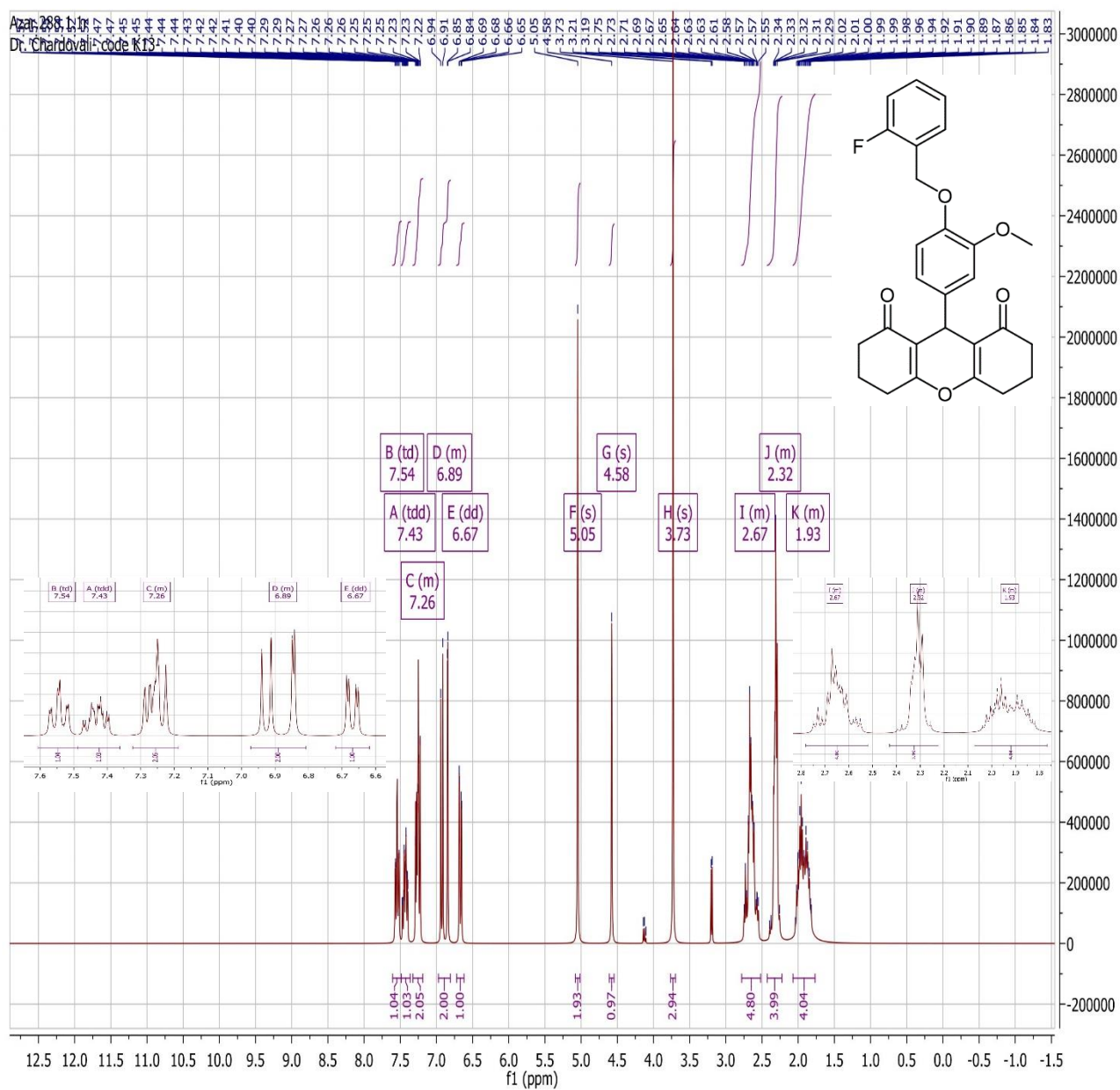
1 H-NMR spectrum of 4m
