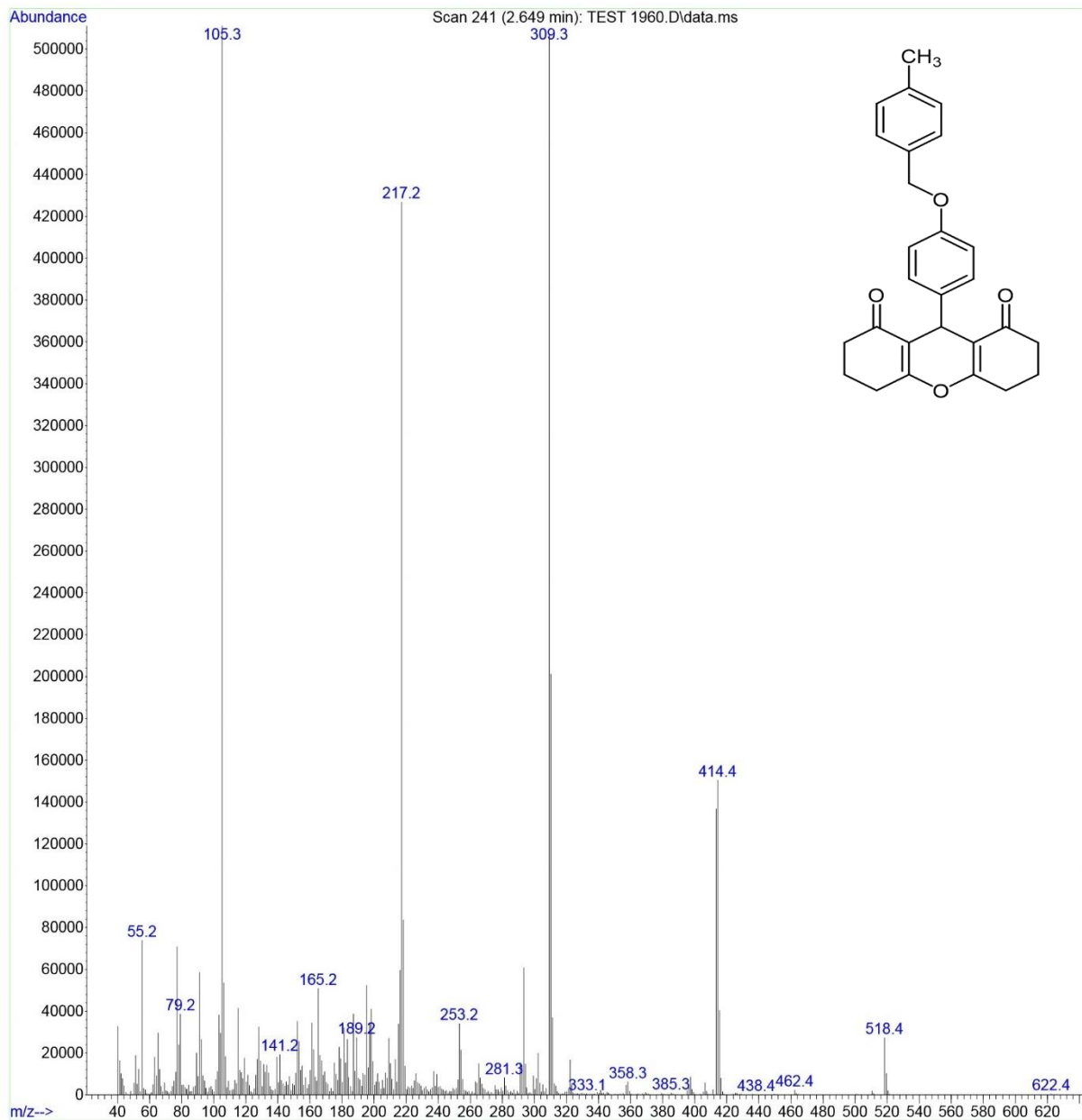
Mass spectrum of 4g
