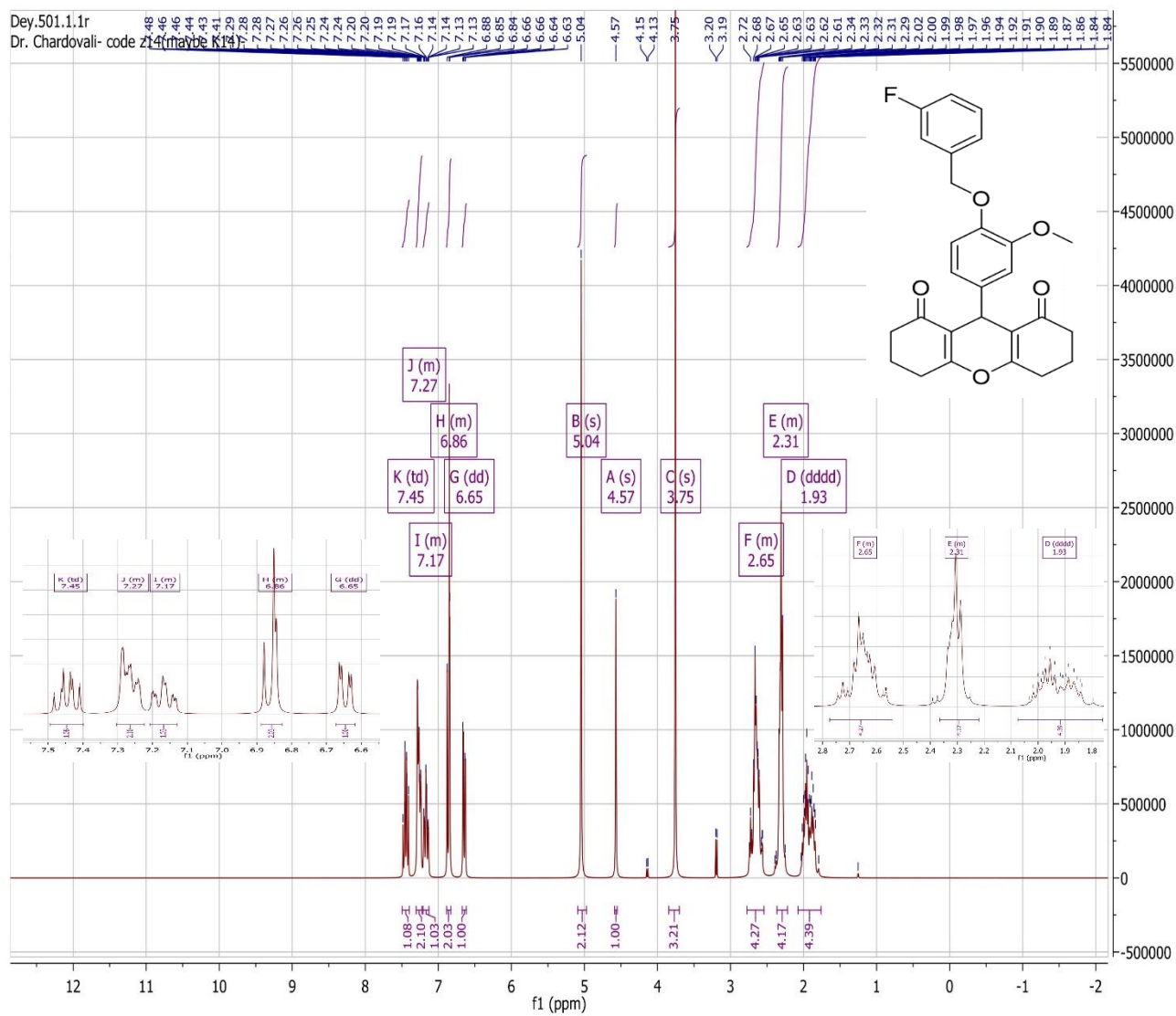
1 H-NMR spectrum of 4n
