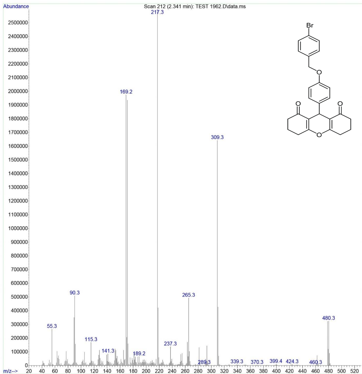
Mass spectrum of 4b
