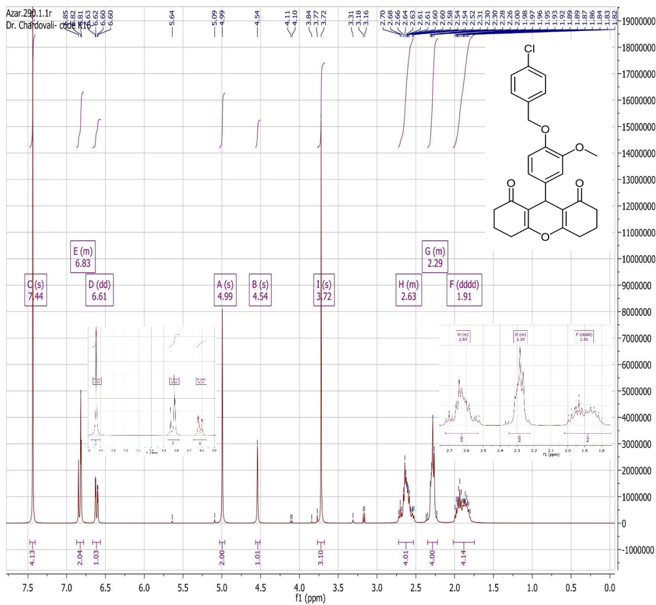
1 H-NMR spectrum of 4p
