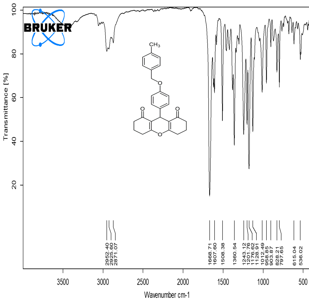
IR spectrum of 4g
