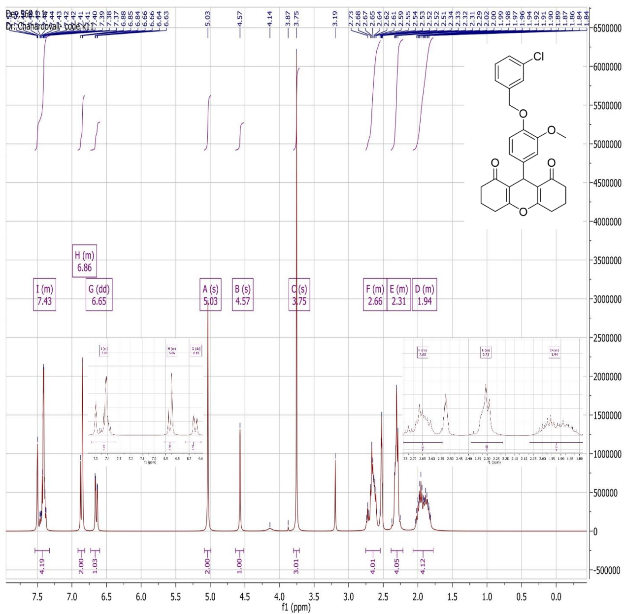
1 H-NMR spectrum of 4k
