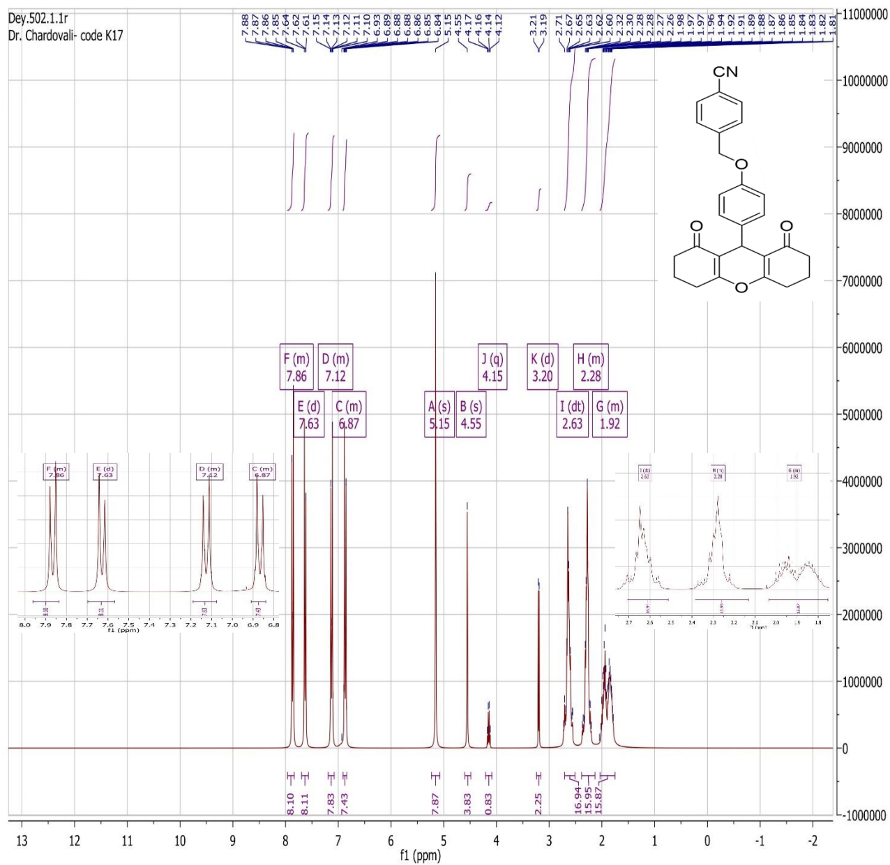
1 H-NMR spectrum of 4q
