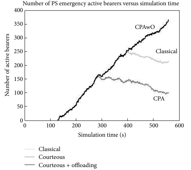
FIGURE 4: Number of PS emergency active bearers.
