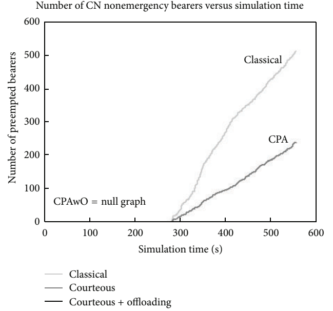
FIGURE 11: Number of CN nonemergency preempted bearers.
