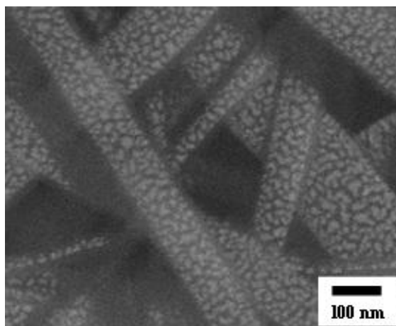
Figure S1. Backscattering electron image of nanofiber thinner than 50 nm in diameter incidentally formed in AuNF100.
