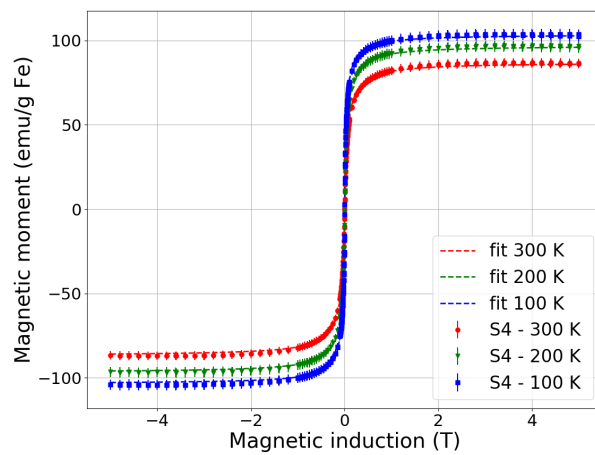
Figure S1: MB curves from -5 T to 5 T for S4 with lognormal distribution fitting.
