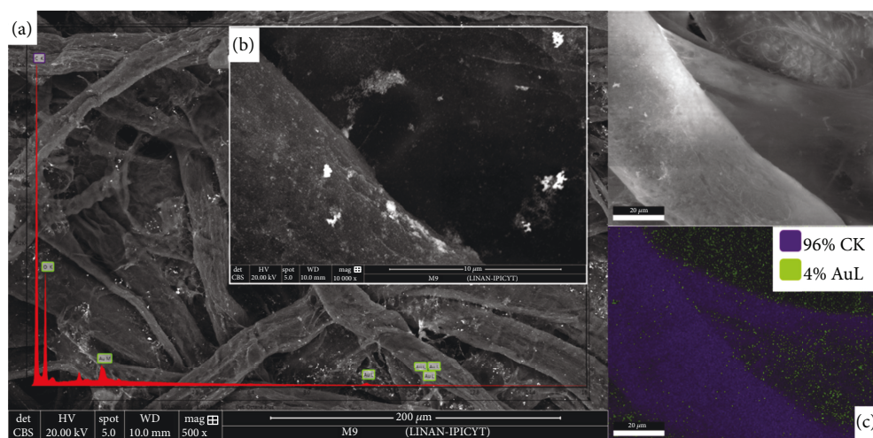
FIGURE 7: FESEM images at different magnifications (a, b) of the surface of cellulose fibers coated with Au biogenic nanoparticles. The inset shows the EDS spectrum collected in (b). (c) Elemental mapping of the Au/biocomposite showing the distribution of Au nanoparticles.
