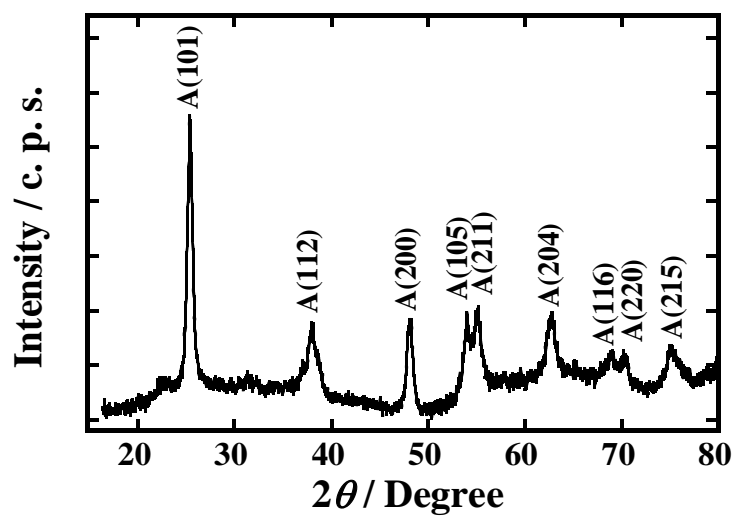
Figure S1. XRD pattern of \text{TiO}_2 nanofibers with the indicate lattice planes corresponding to anatase phase
