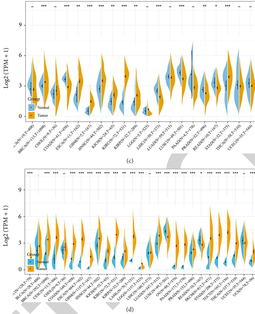
FIGURE 1: IL2RB expression in pan-cancer. (a) Expression levels of IL2RB in a database contain 31 tissues, obtained from the GTEx. (b) Expression levels of IL2RB in a dataset containing 21 tissues in tumor cell lines, collected from the CCLE. (c) Expression levels of ATG5 in tumor and paired adjacent noncancerous tissues containing 20 tissues from TCGA, * P < 0.05 , ** P < 0.01 , and *** P < 0.001 . (d) IL2RB expression difference in 27 tumors integrating data of normal tissues in GTEx database and data of TCGA tumor tissues, * P < 0.05 , ** P < 0.01 , and *** P < 0.001 .
