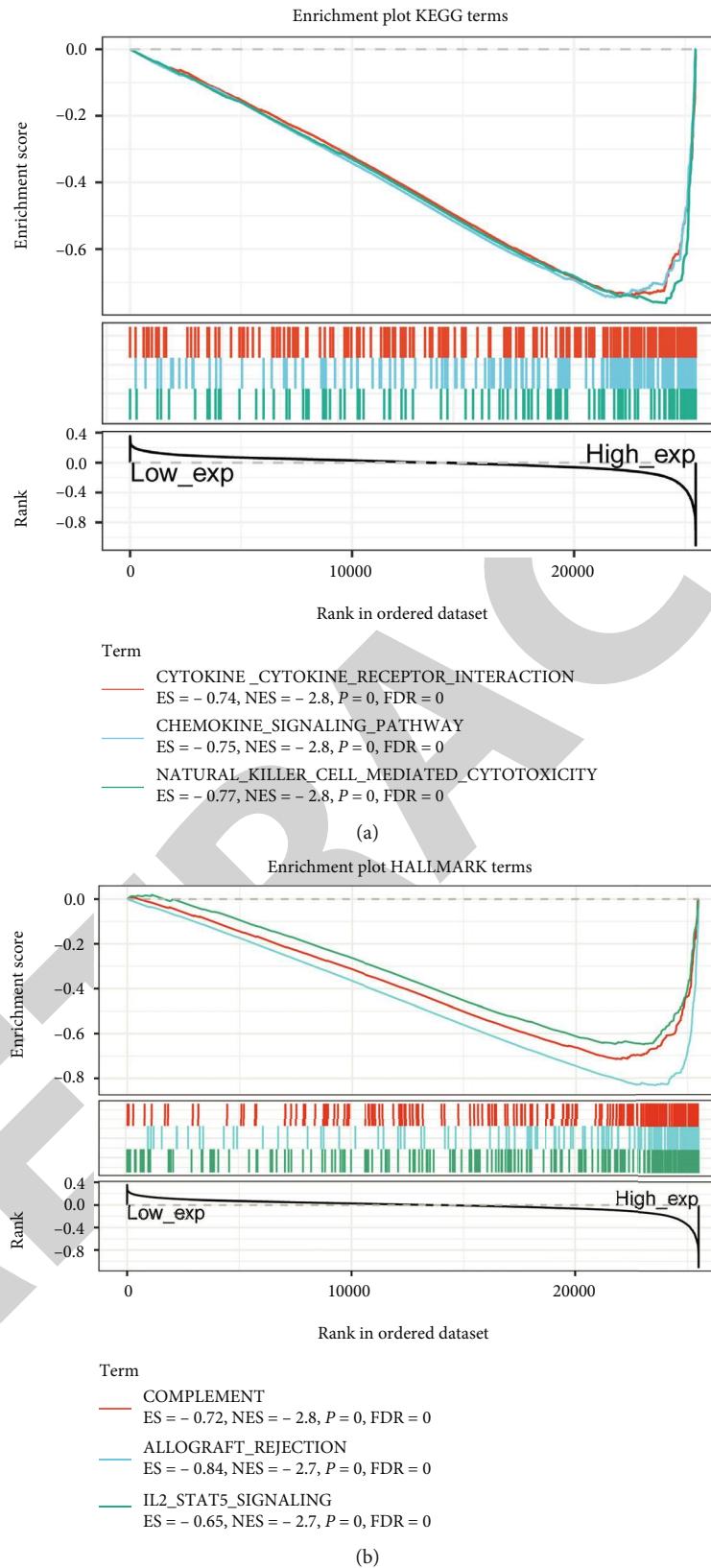
FIGURE 12: Gene set enrichment analysis of IL2RB associated with signaling pathways in KEGG and hallmark datasets. (a) Results of GSEA of IL2RB ranked in the top 3 for its association with signaling pathways in KEGG database. (b) Results of GSEA of the top 3 rankings of IL2RB correlation with signaling pathways in hallmark dataset.
