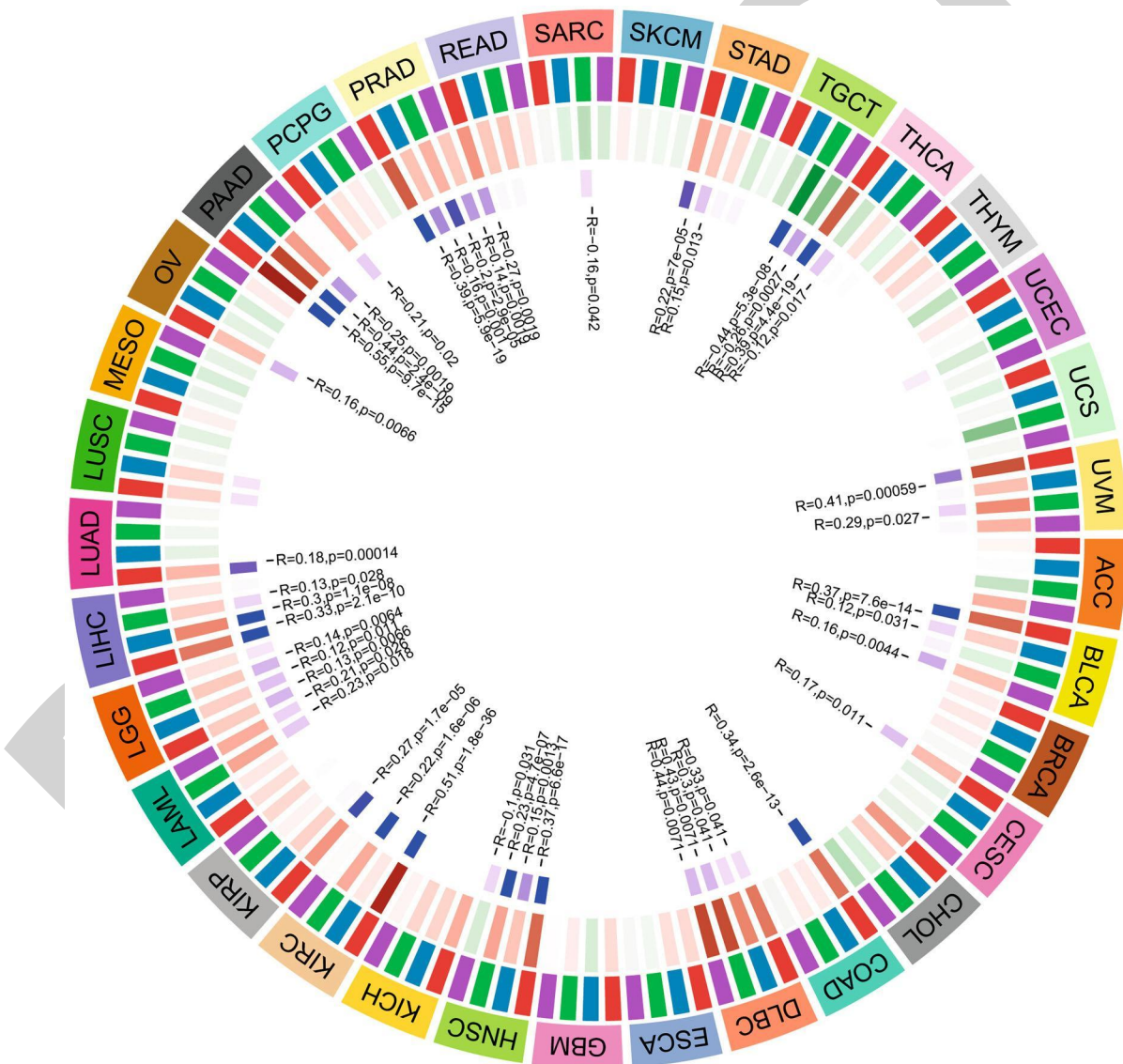
FIGURE 11: Correlation analysis between the expression of IL2RB in pan-cancer and the expression levels of four types of methyltransferases. DNMT1 is colored red, DNMT2 was colored blue, DNMT3a was colored green, and DNMT3b is colored purple.
