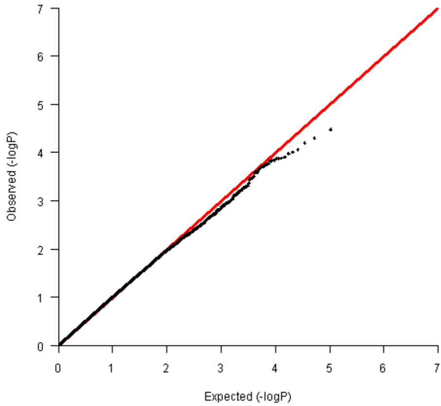
Supplementary Figure 1. Q-Q plot of logistic regression models adjusted for age, gender, diabetes duration and HbA1C level.
