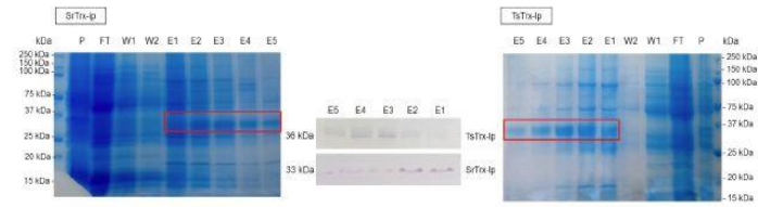
SUPPLEMENTARY FIGURE 1: Coomassie-stained SDS-PAGE of purification steps of recombinant SrTrx-lp (left) and TsTrx-lp (right) as well as Western Blot analysis (middle) of both eluted proteins. Elutions (E1-E5) were distinct lines at approximately 33 kDa (SrTrx-lp) and 36 kDa (TsTrx-lp). P: pellet; FT: flow through; W1: wash step 1; W2: wash step 2.
