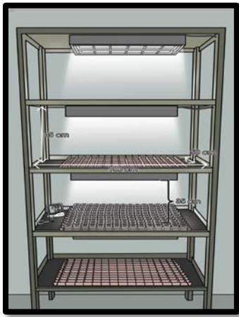
Supplemental Figure 1. Illuminated cabinet devised and used for cercarial emergence. Distance of light source to the top surface of the specimen container is 35 cm. Set-up includes apparatus for temperature and relative humidity determination and a lux meter for measuring light intensity.
