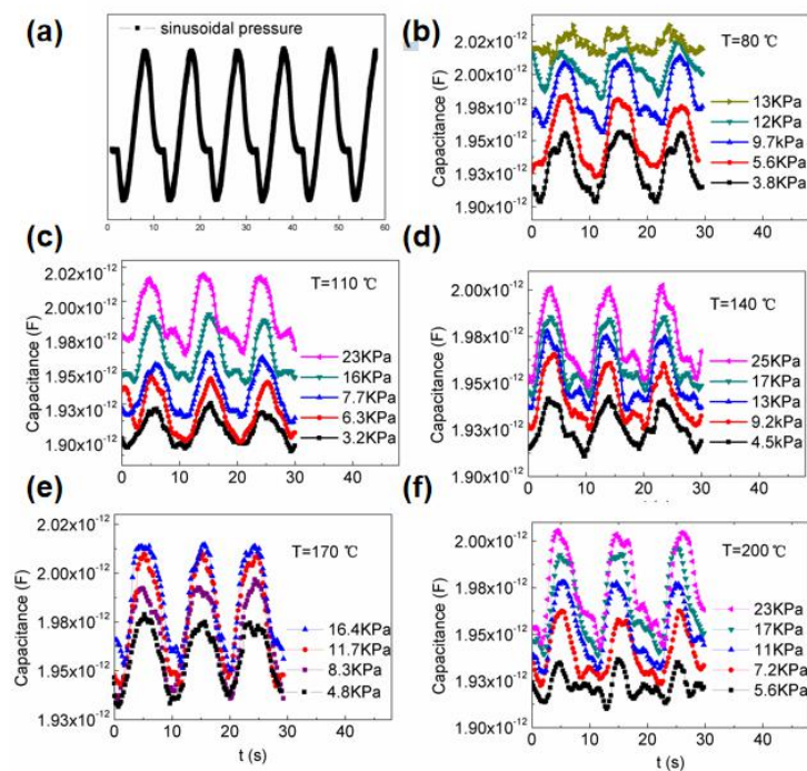
Supplementary Figure S1. (a) The waveform of 0.1 Hz sinusoidal pressure generated by vibration exciter. The corresponding capacitance changing characteristics of PDMS capacitor under (b) 80°C, (c) 110°C, (d) 140°C, (e) 170°C, (f) 200°C.
