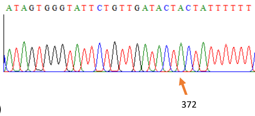
Figure S1. An example of visual conformation of nucleotide substitution. (a) Main haplotype sequence H3 showing G at site 372. (b) A derived haplotype H36 (H3_372G>A), showing A at site 372.
