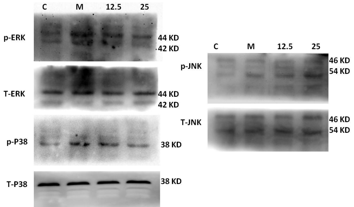
Figure 1 Full bolt figure of MAPK pathways effected by TIE
