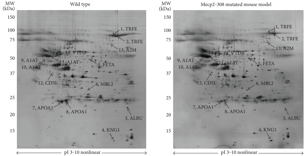
FIGURE 1: Silver-stained 2-DE of proteins from wild-type and Mecp2 -308 mutated mouse models. A total of 60 \mu g of protein from albumin-depleted plasma samples was subjected to the first dimension electrophoresis on IPG strips, with nonlinear pH ranging from 3 to 10 (pI, isoelectric point), followed by SDS-polyacrylamide gradient gel (8–16% T) electrophoresis. Molecular mass (MW, kDa) and pI markers are indicated along the gels. Numbers followed by short names denote the mass spectrometry-identified protein spots listed in Tables 1 and 2.
