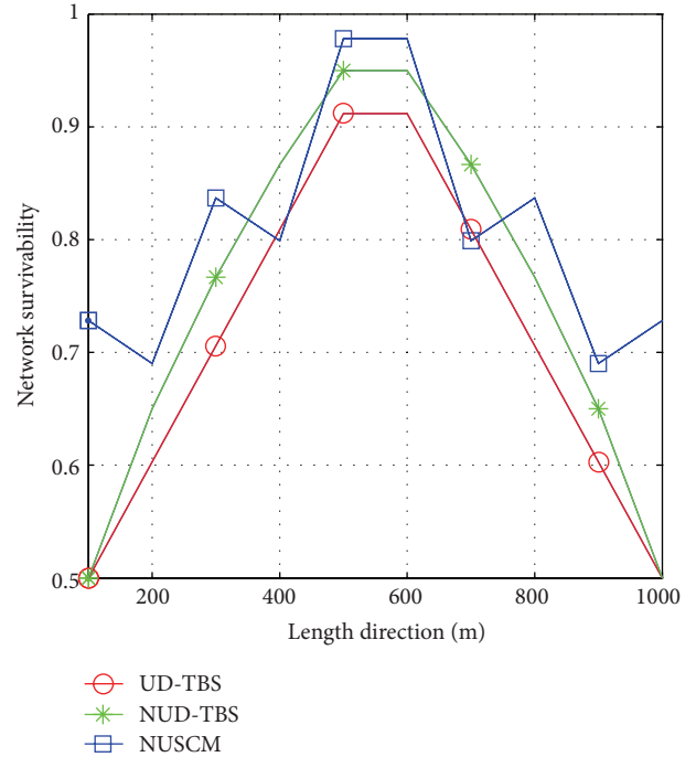
FIGURE 10: Network survivability.
