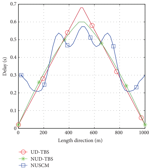
FIGURE 11: Data delay.
