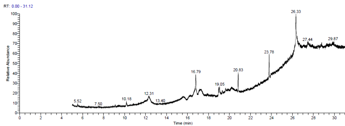
S1. Fig.1. Chromatogram of GC-MS analysis of S. persica extract
