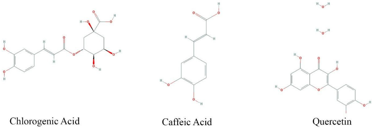
Figure S2: Molecules Structures of Phenolic Compounds.
