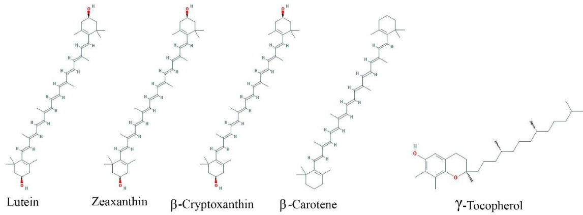
Figure S1: Molecules Structures of Carotenoides.
