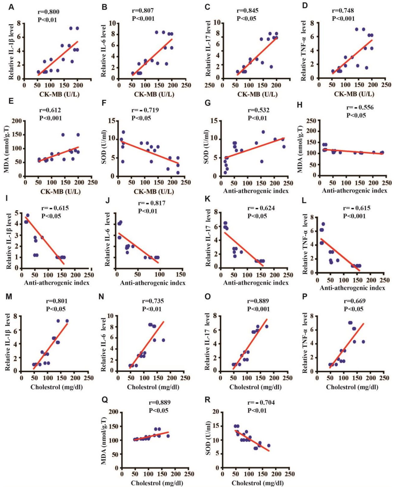
Fig. 1: Correlations between CK-MB, anti-atherogenic index and cholesterol with IL-1 \beta , IL-6, IL-17, TNF- \alpha , MDA and SOD among high-fat diet feeding rats
