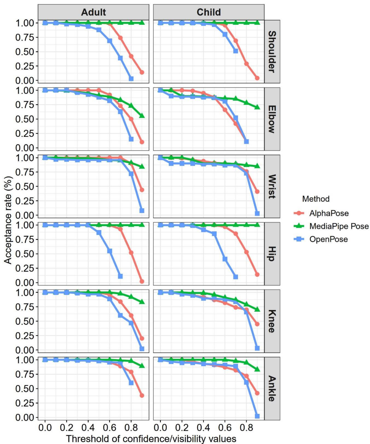
Figure S1. Acceptance rate of each pose estimation method for each keypoint.
