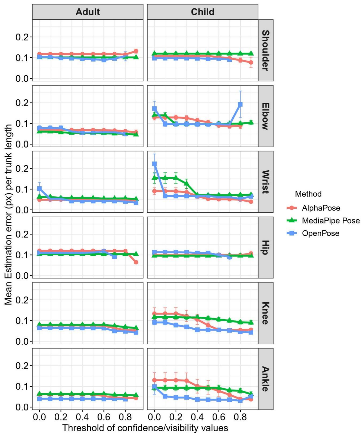
Figure S2. Estimation error distance of each pose estimation method for each keypoint.
