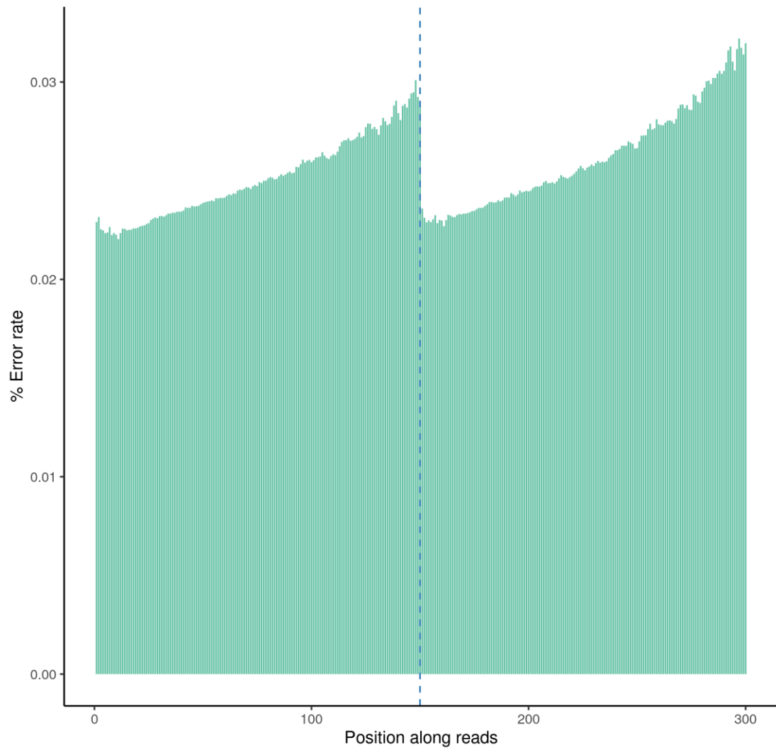
Error rate distribution along reads ( N2 )
