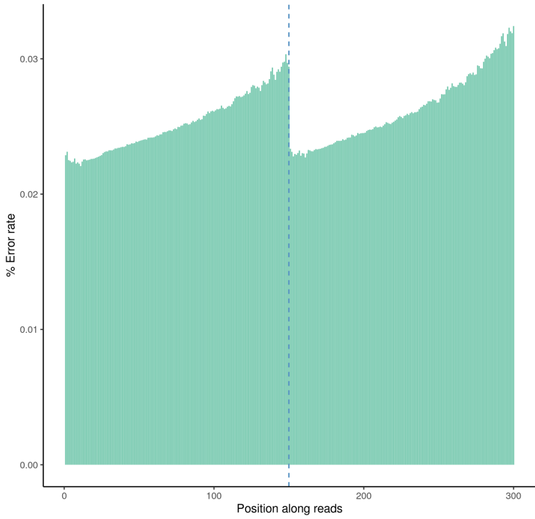
Error rate distribution along reads ( M1 )
