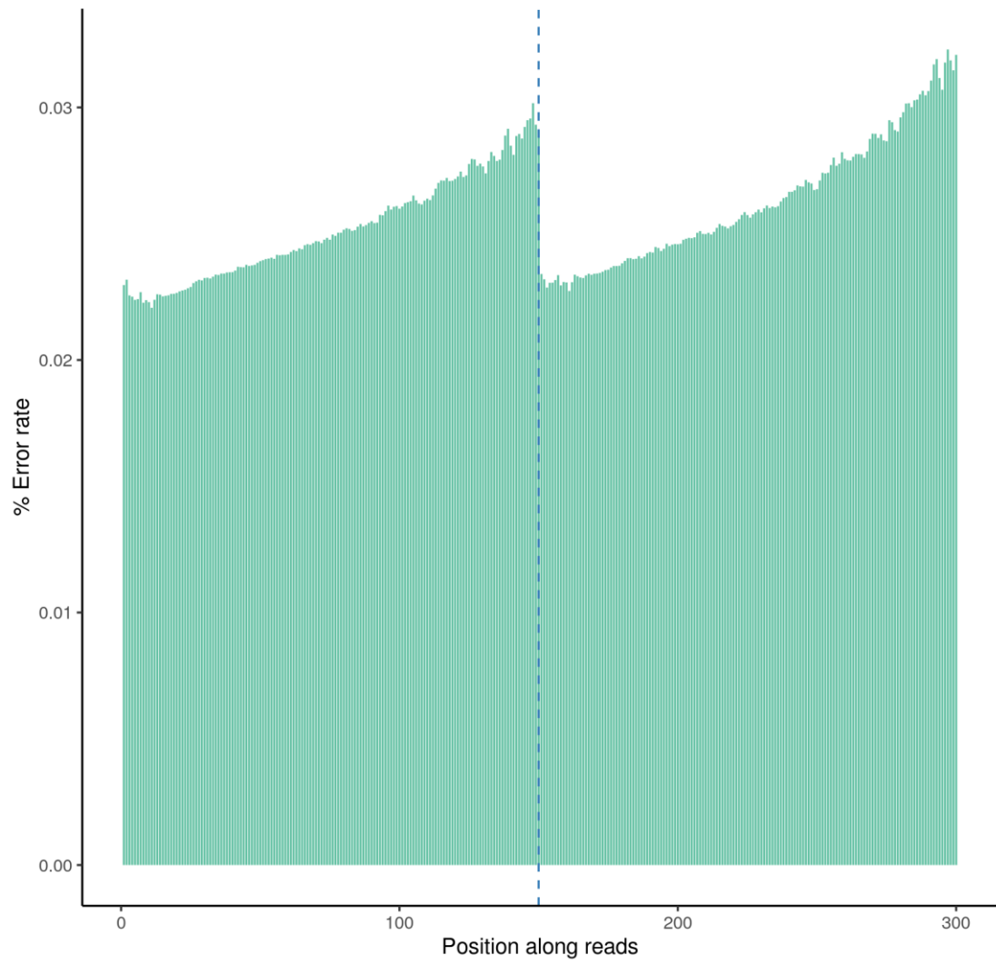
Error rate distribution along reads ( N3 )
