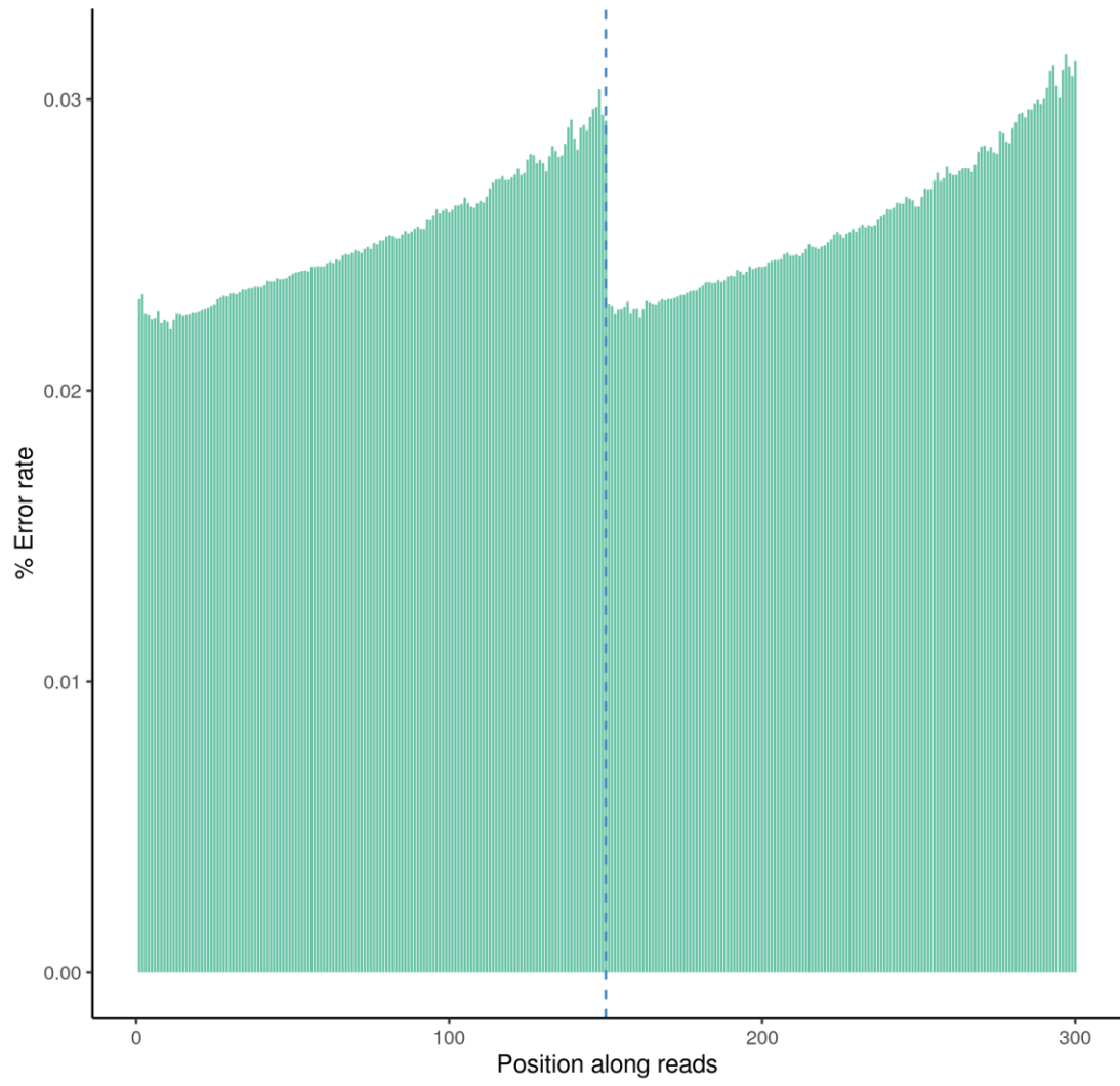
Error rate distribution along reads ( N1 )
