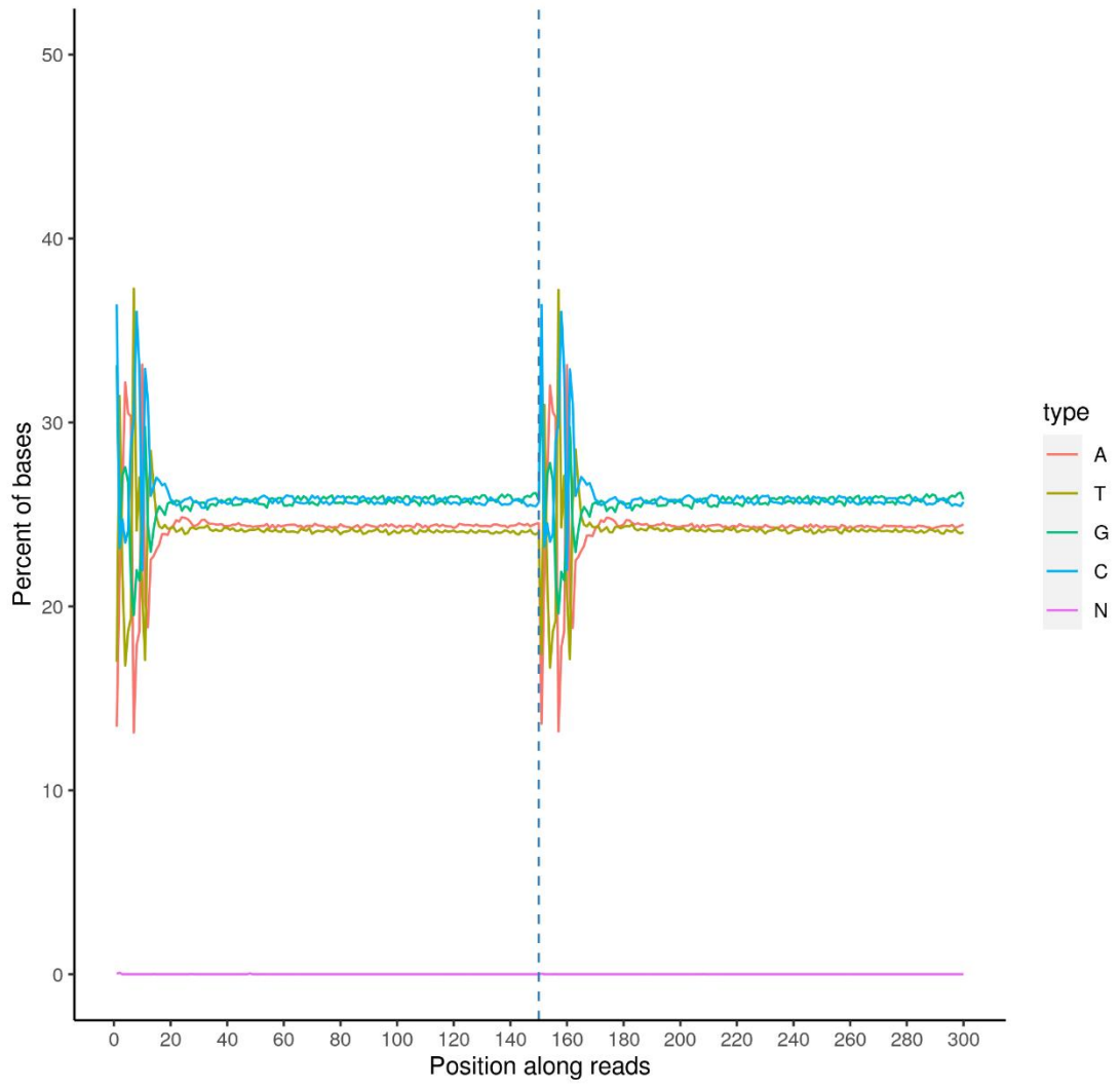
Bases content along reads ( M1 )
