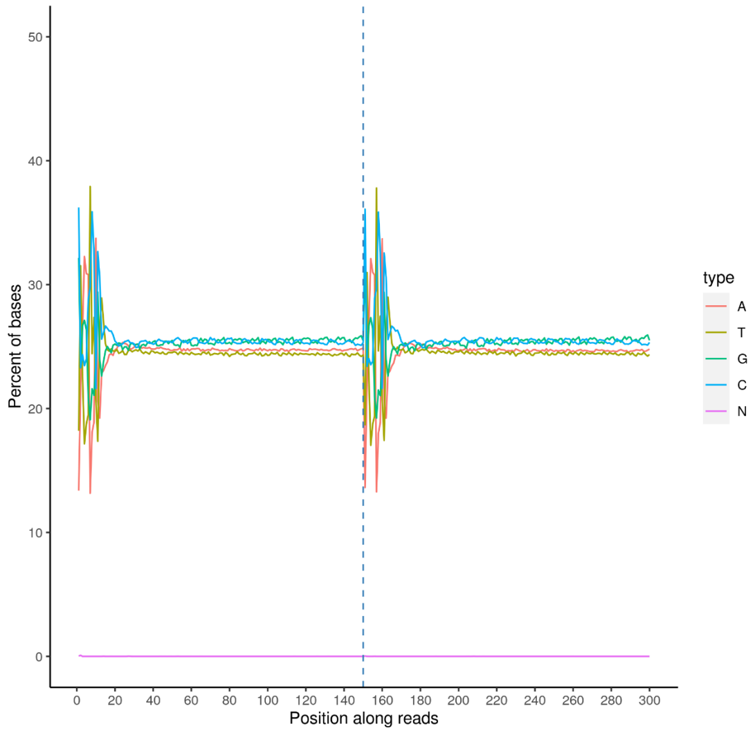
Bases content along reads ( M3 )
