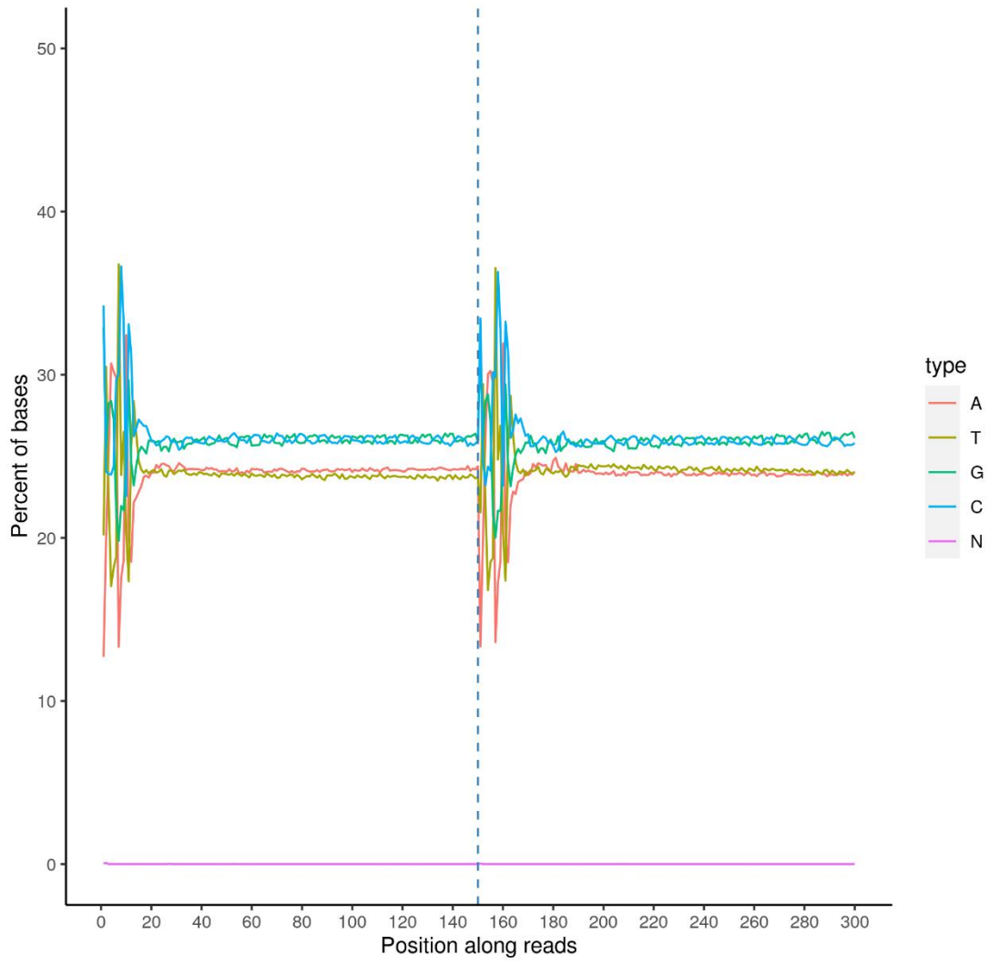
Bases content along reads ( M2 )
