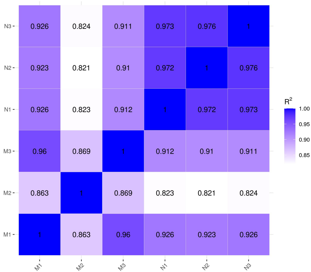
Pearson correlation between samples
