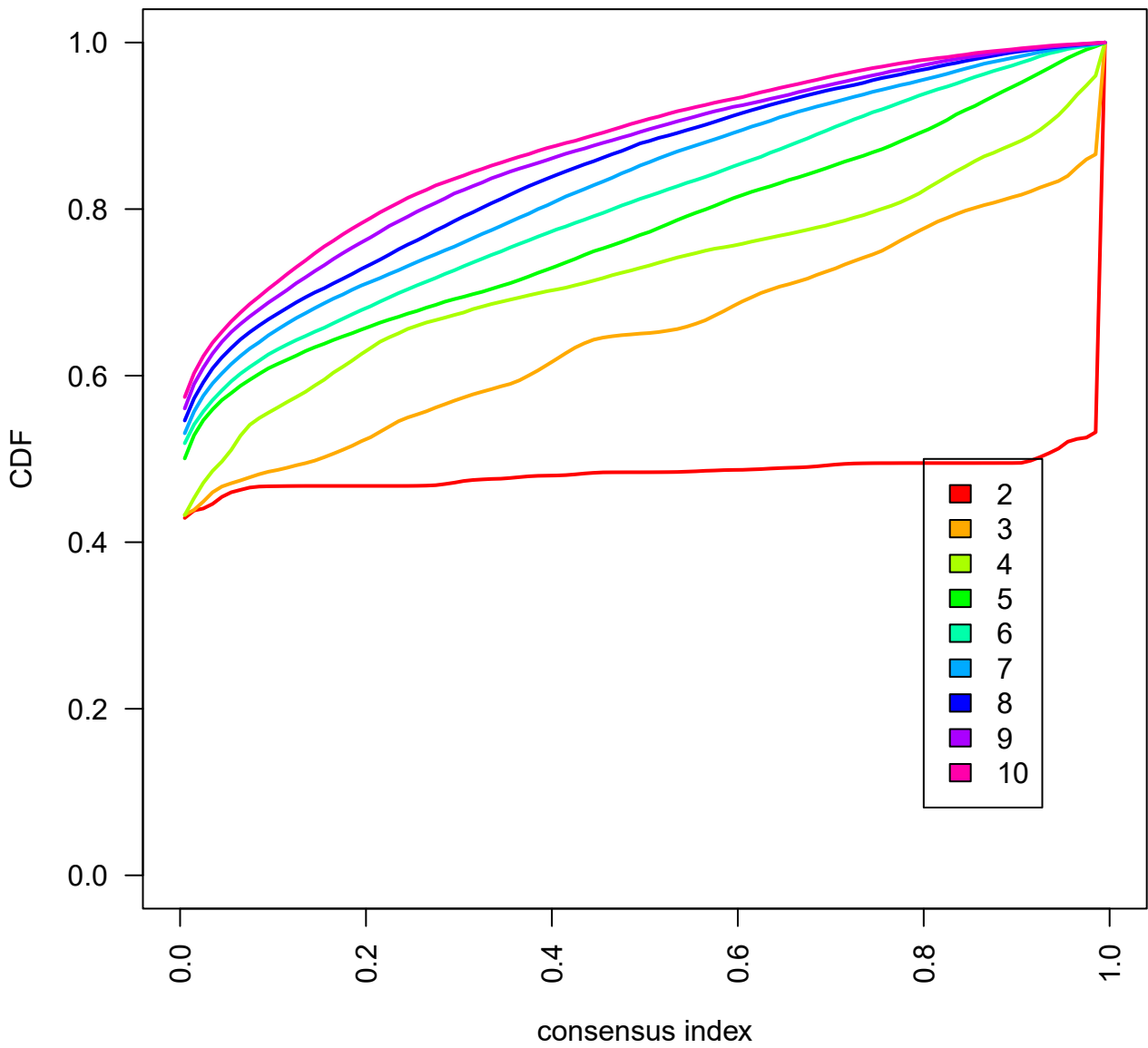
consensus CDF
