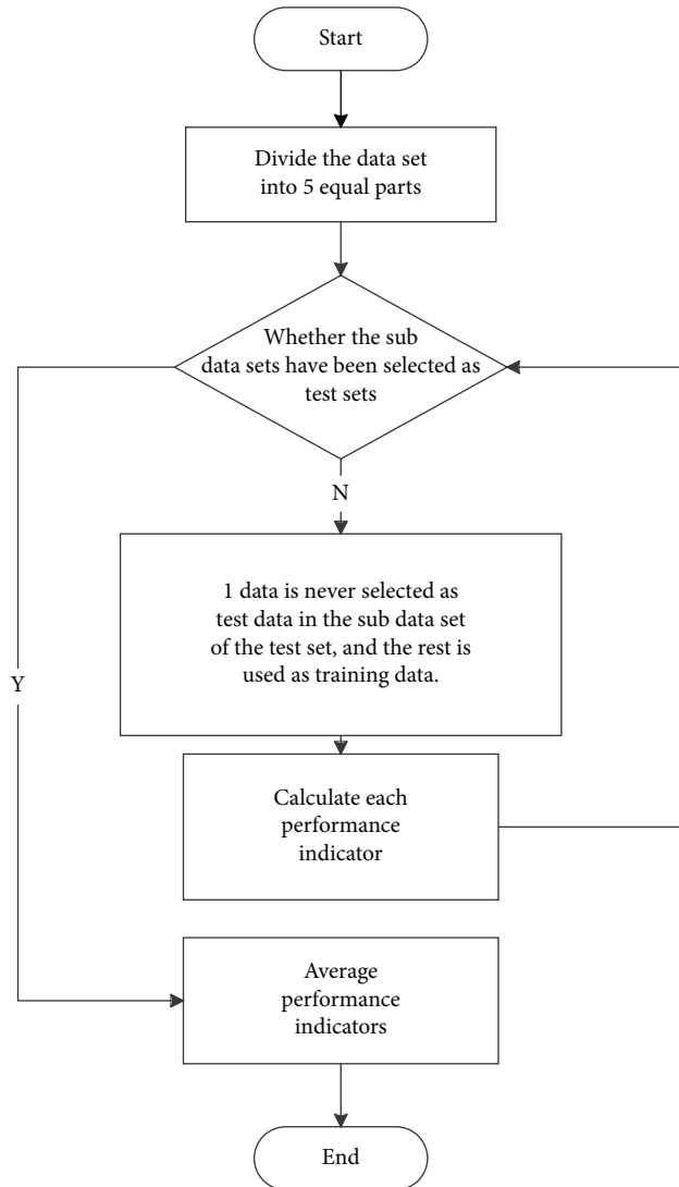
FIGURE 3: Flow chart of the five-fold algorithm.
