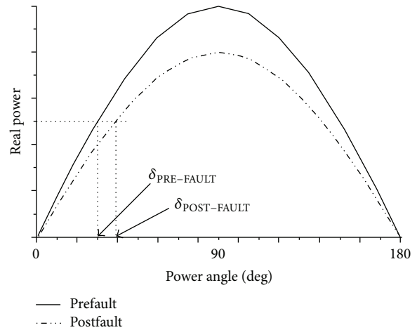
FIGURE 4: Power transfer between two buses.
