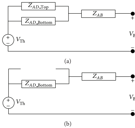
FIGURE 3: Thevenin equivalent circuit illustrating the fault process: (a) prefault operation and (b) postfault operation.
