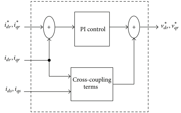
FIGURE 5: Conventional (indirect) current regulator.
