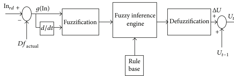
FIGURE 6: Block diagram of fuzzy controller.
