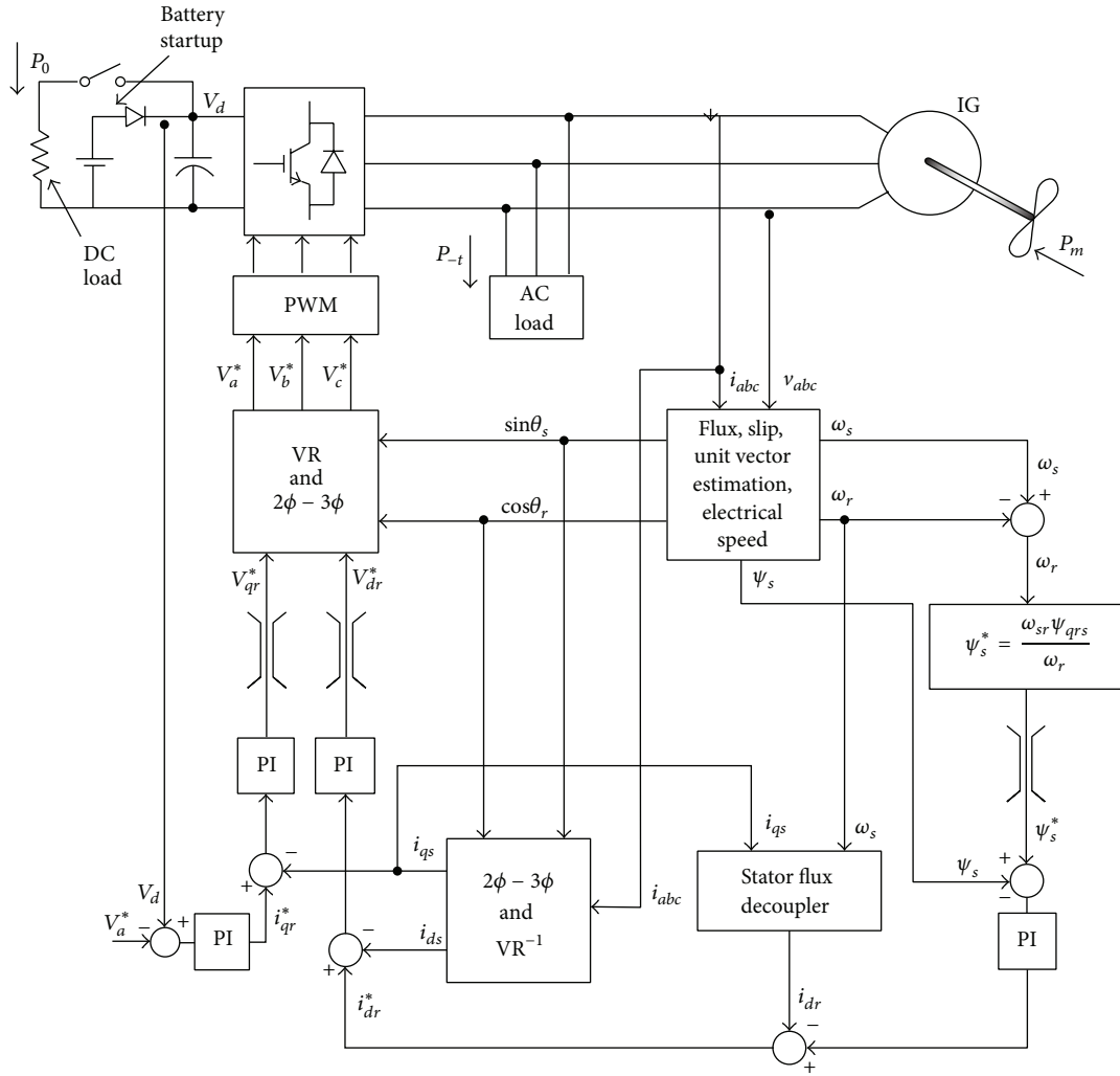
FIGURE 1: DFIG wind turbine.
