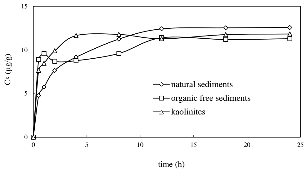
Figure S1. Sorption kinetic of phenanthrene on 3 sorbents
